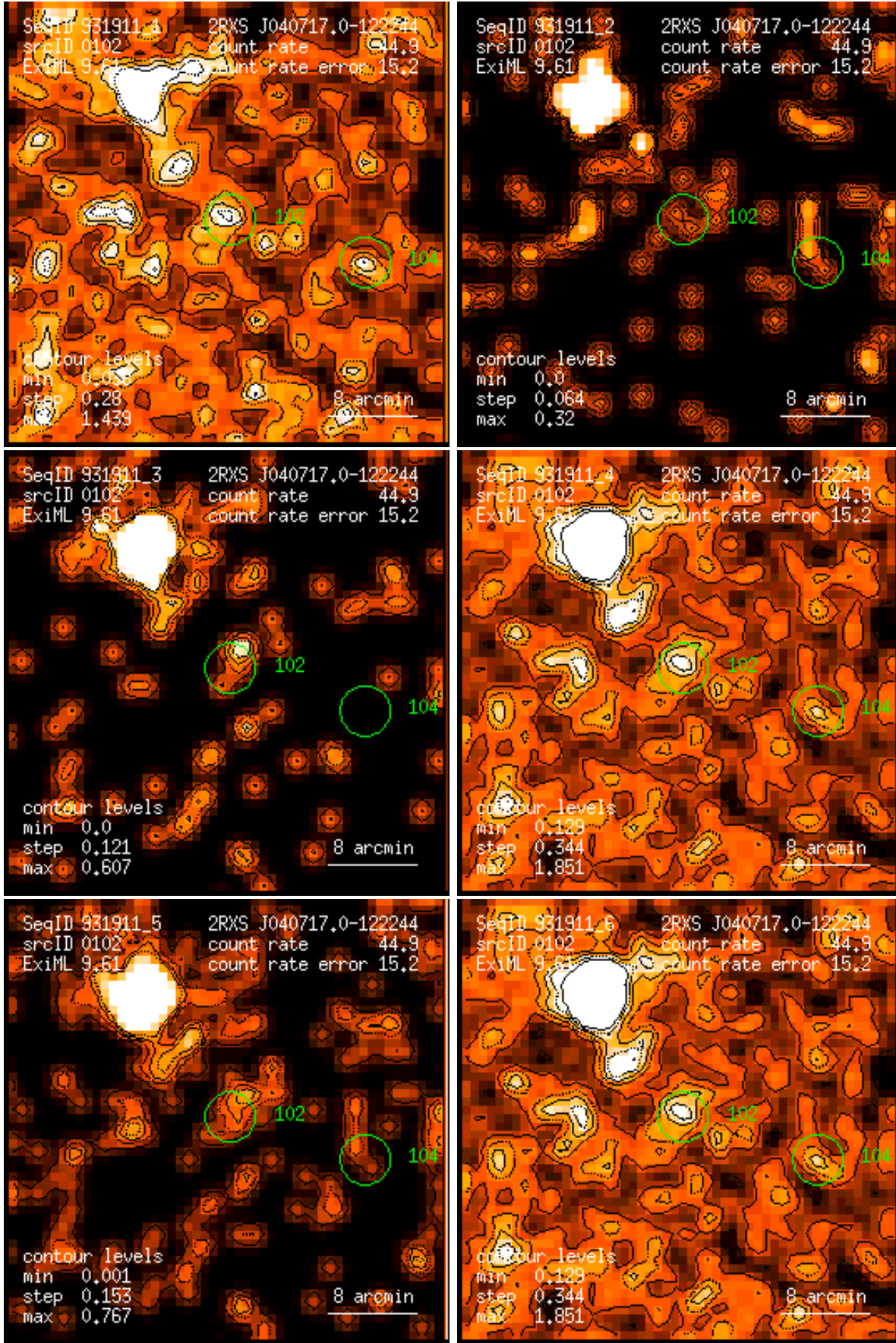
Figure 102: RASS 931911: detection 0102: band rate images, Gaussian filter: (1) PSPC channels 11 – 41, (2) 52 – 90, (3) 91 – 201, (4) 11 – 235, (5) 52 – 201, (6) 11 – 201. Broad band rates in counts/ks. Band rate contour levels in counts/ks/arcmin 2 .
