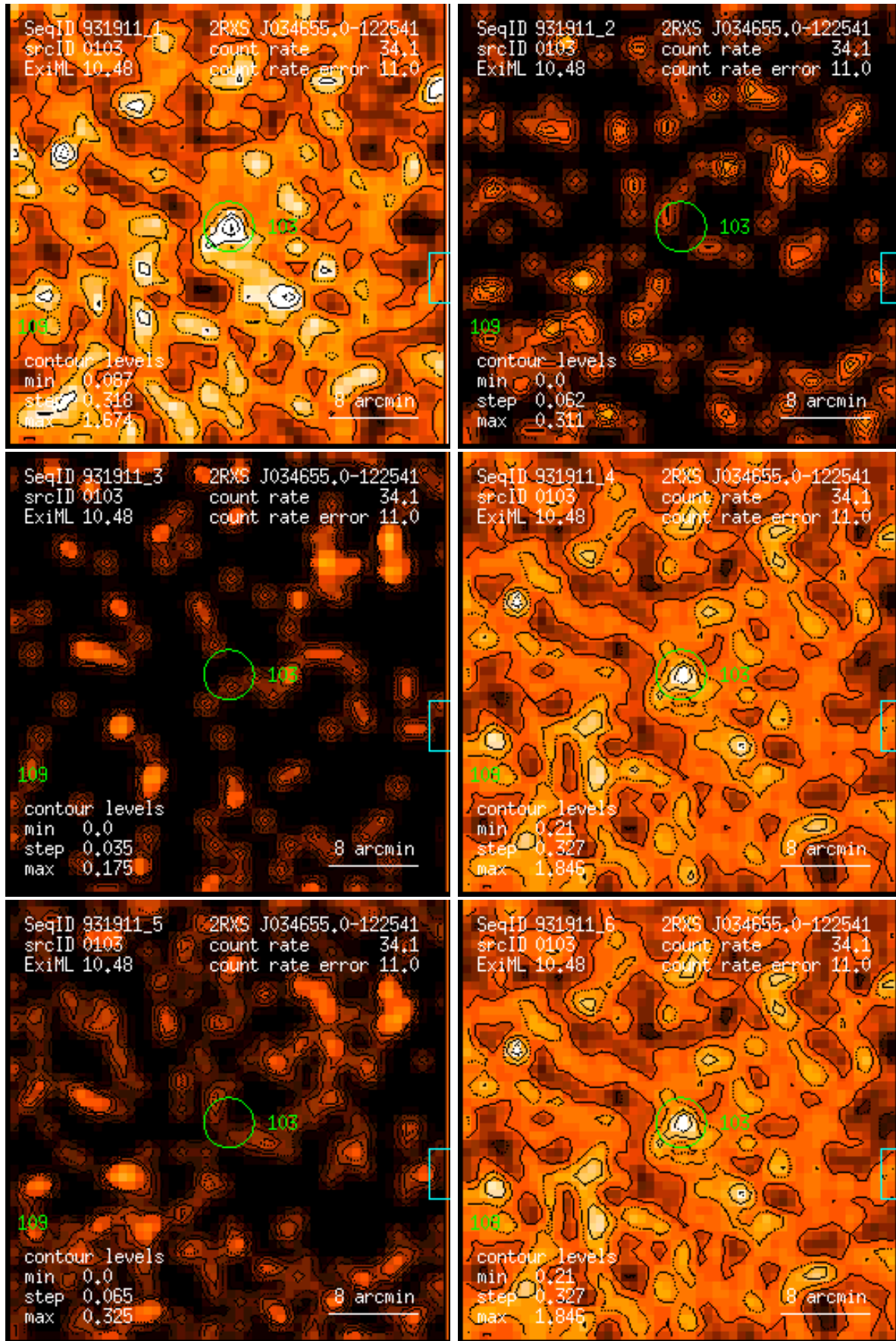
Figure 103: RASS 931911: detection 0103: band rate images, Gaussian filter: (1) PSPC channels 11 – 41, (2) 52 – 90, (3) 91 – 201, (4) 11 – 235, (5) 52 – 201, (6) 11 – 201. Broad band rates in counts/ks. Band rate contour levels in counts/ks/arcmin 2 .
