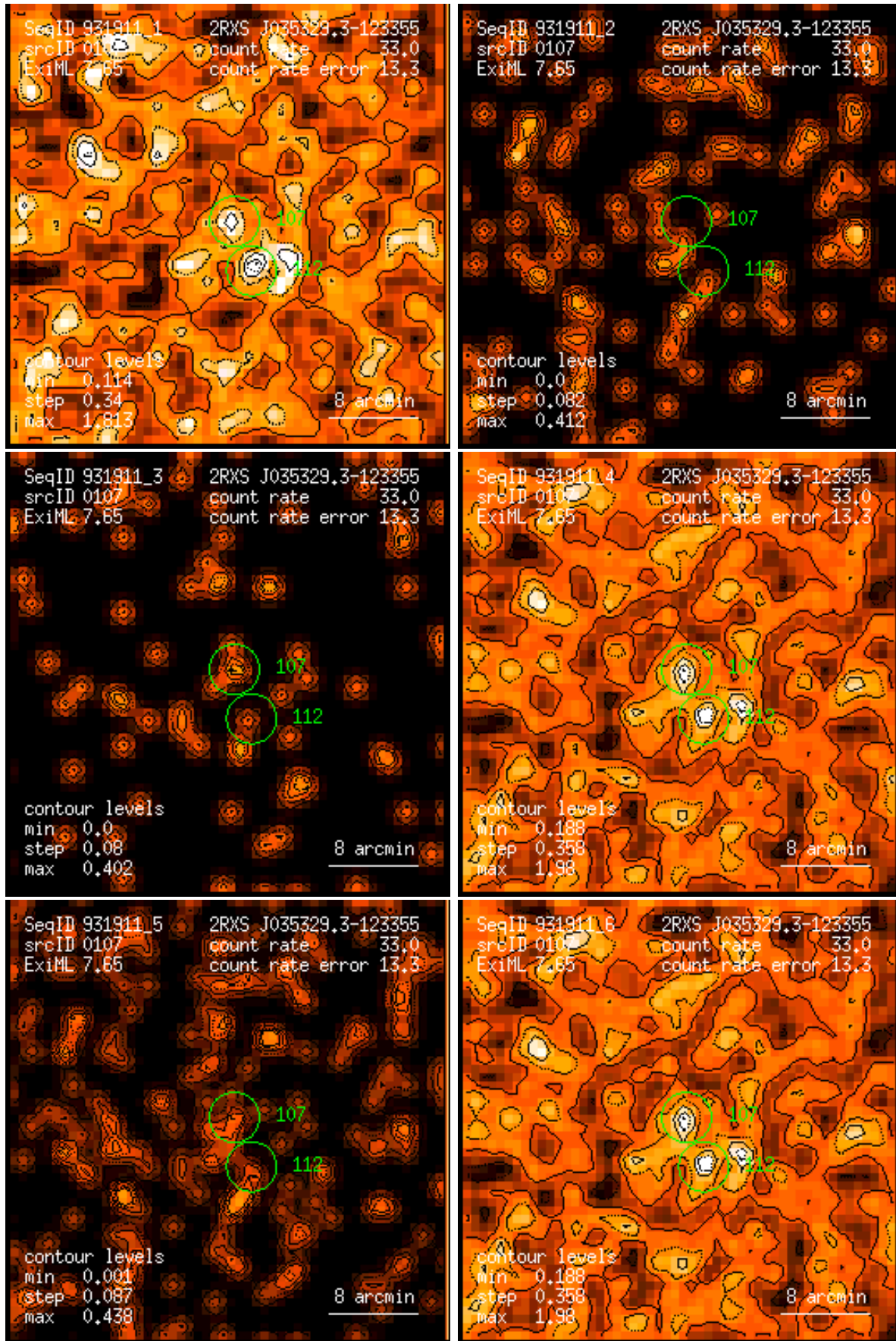
Figure 107: RASS 931911: detection 0107: band rate images, Gaussian filter: (1) PSPC channels 11 – 41, (2) 52 – 90, (3) 91 – 201, (4) 11 – 235, (5) 52 – 201, (6) 11 – 201. Broad band rates in counts/ks. Band rate contour levels in counts/ks/arcmin 2 .
