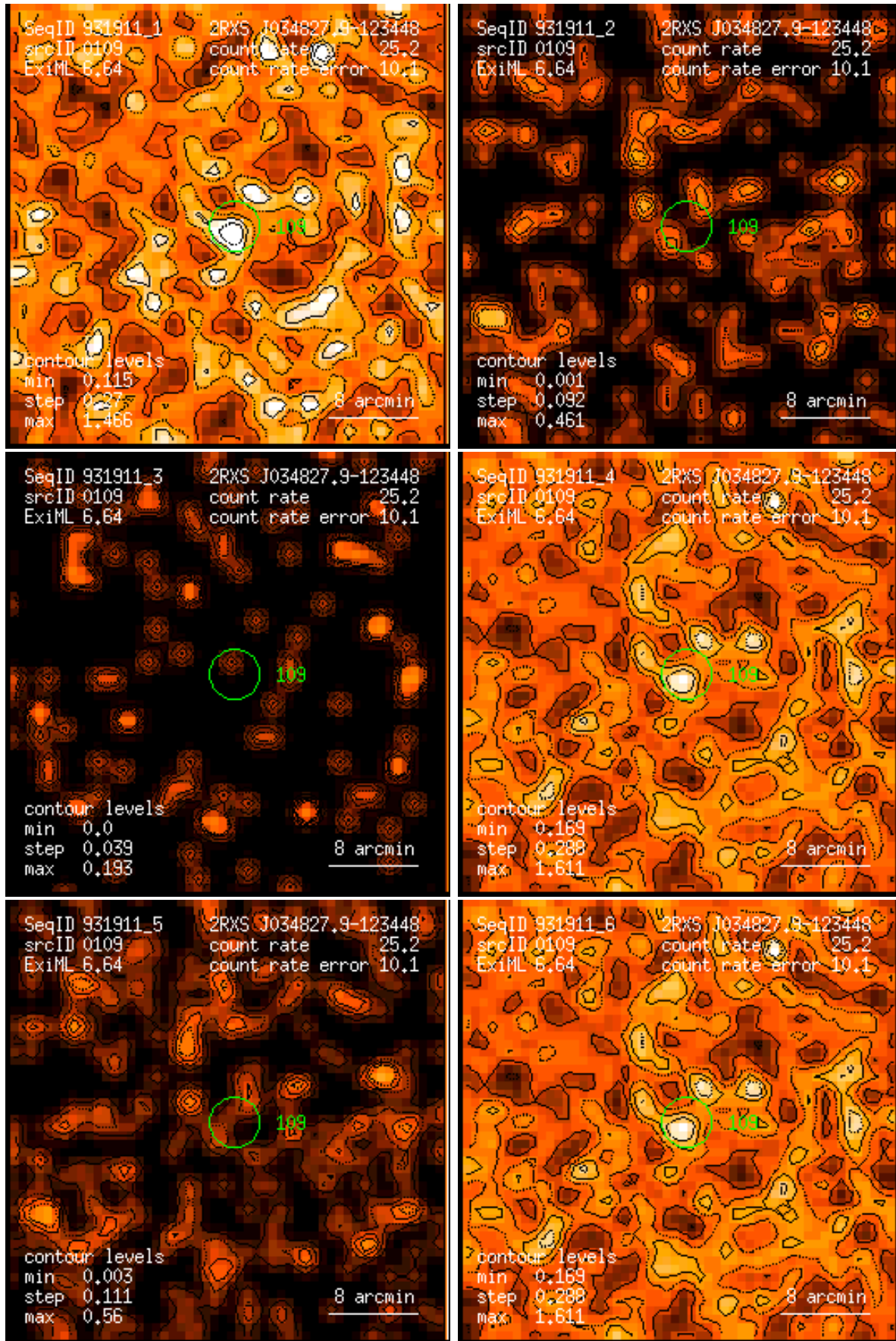
Figure 109: RASS 931911: detection 0109: band rate images, Gaussian filter: (1) PSPC channels 11 – 41, (2) 52 – 90, (3) 91 – 201, (4) 11 – 235, (5) 52 – 201, (6) 11 – 201. Broad band rates in counts/ks. Band rate contour levels in counts/ks/arcmin 2 .
