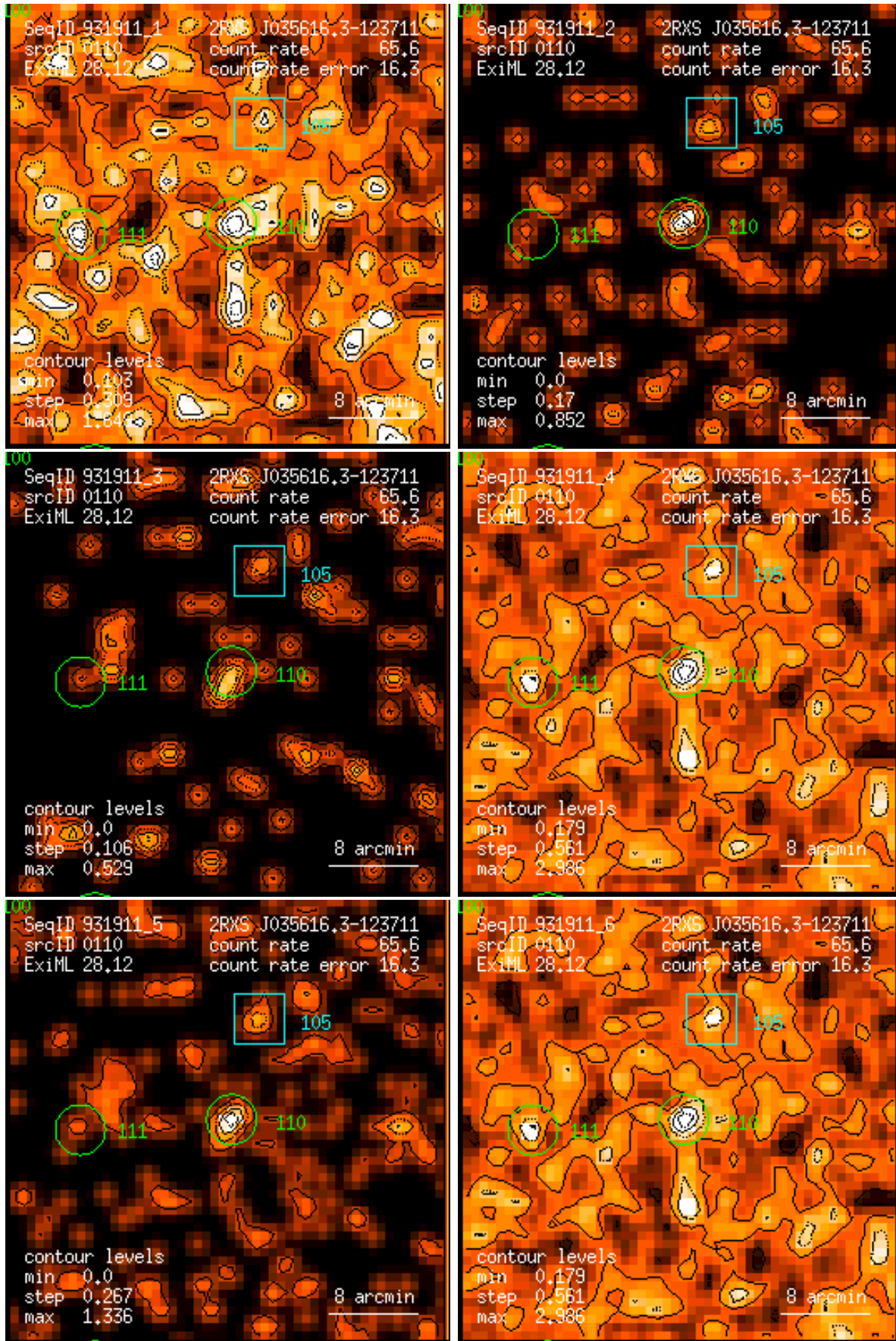
Figure 110: RASS 931911: detection 0110: band rate images, Gaussian filter: (1) PSPC channels 11 – 41, (2) 52 – 90, (3) 91 – 201, (4) 11 – 235, (5) 52 – 201, (6) 11 – 201. Broad band rates in counts/ks. Band rate contour levels in counts/ks/arcmin 2 .
