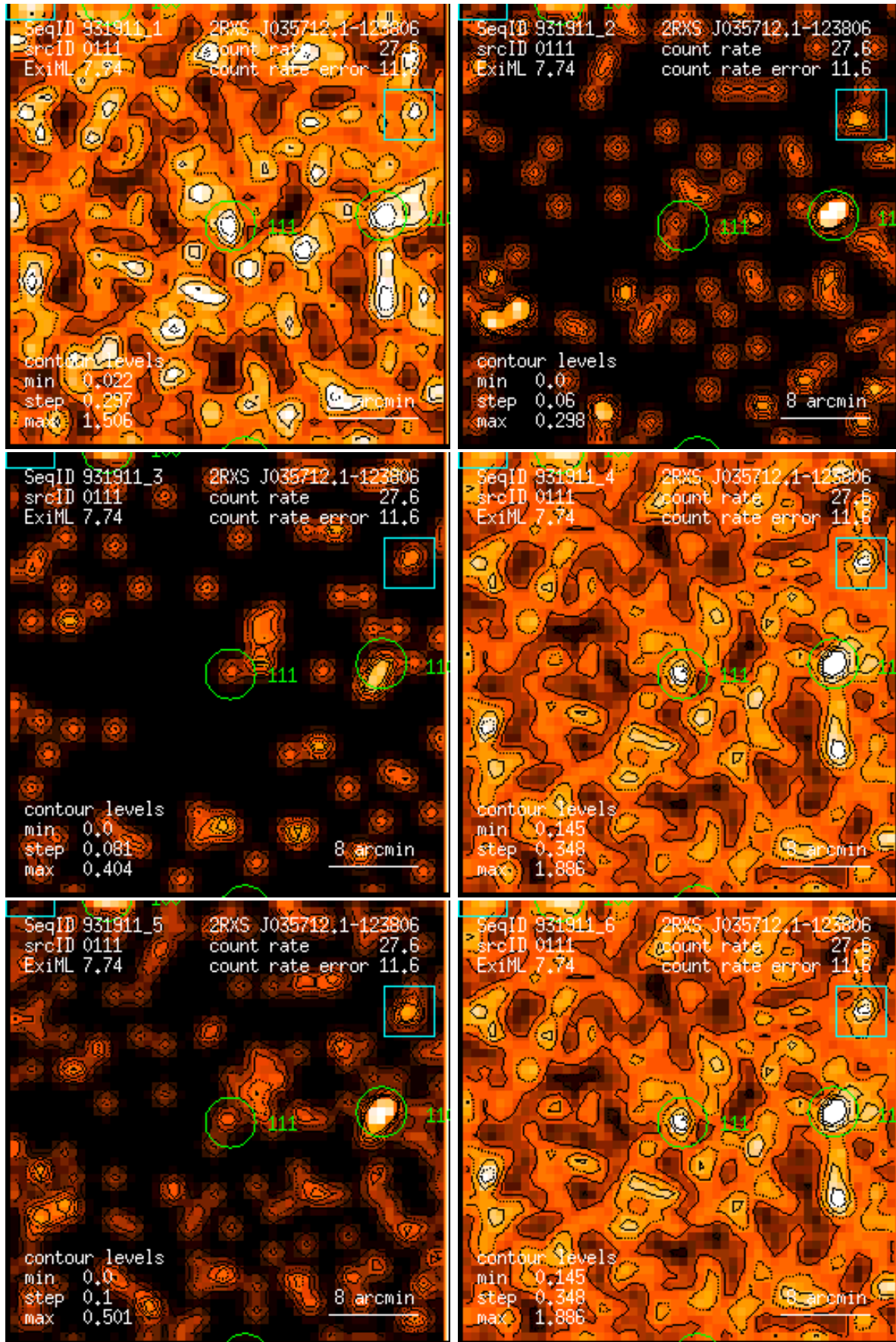
Figure 111: RASS 931911: detection 0111: band rate images, Gaussian filter: (1) PSPC channels 11 – 41, (2) 52 – 90, (3) 91 – 201, (4) 11 – 235, (5) 52 – 201, (6) 11 – 201. Broad band rates in counts/ks. Band rate contour levels in counts/ks/arcmin 2 .
