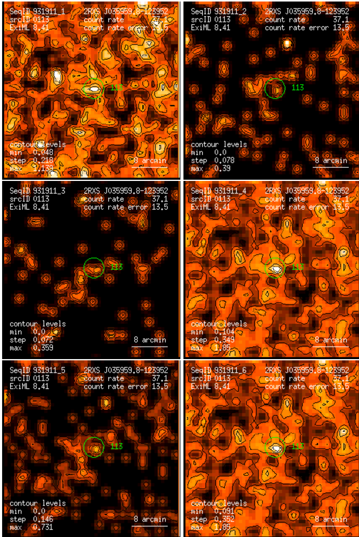
Figure 113: RASS 931911: detection 0113: band rate images, Gaussian filter: (1) PSPC channels 11 – 41, (2) 52 – 90, (3) 91 – 201, (4) 11 – 235, (5) 52 – 201, (6) 11 – 201. Broad band rates in counts/ks. Band rate contour levels in counts/ks/arcmin 2 .
