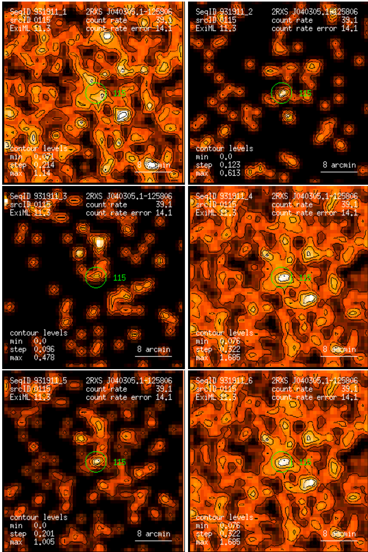
Figure 115: RASS 931911: detection 0115: band rate images, Gaussian filter: (1) PSPC channels 11 – 41, (2) 52 – 90, (3) 91 – 201, (4) 11 – 235, (5) 52 – 201, (6) 11 – 201. Broad band rates in counts/ks. Band rate contour levels in counts/ks/arcmin 2 .
