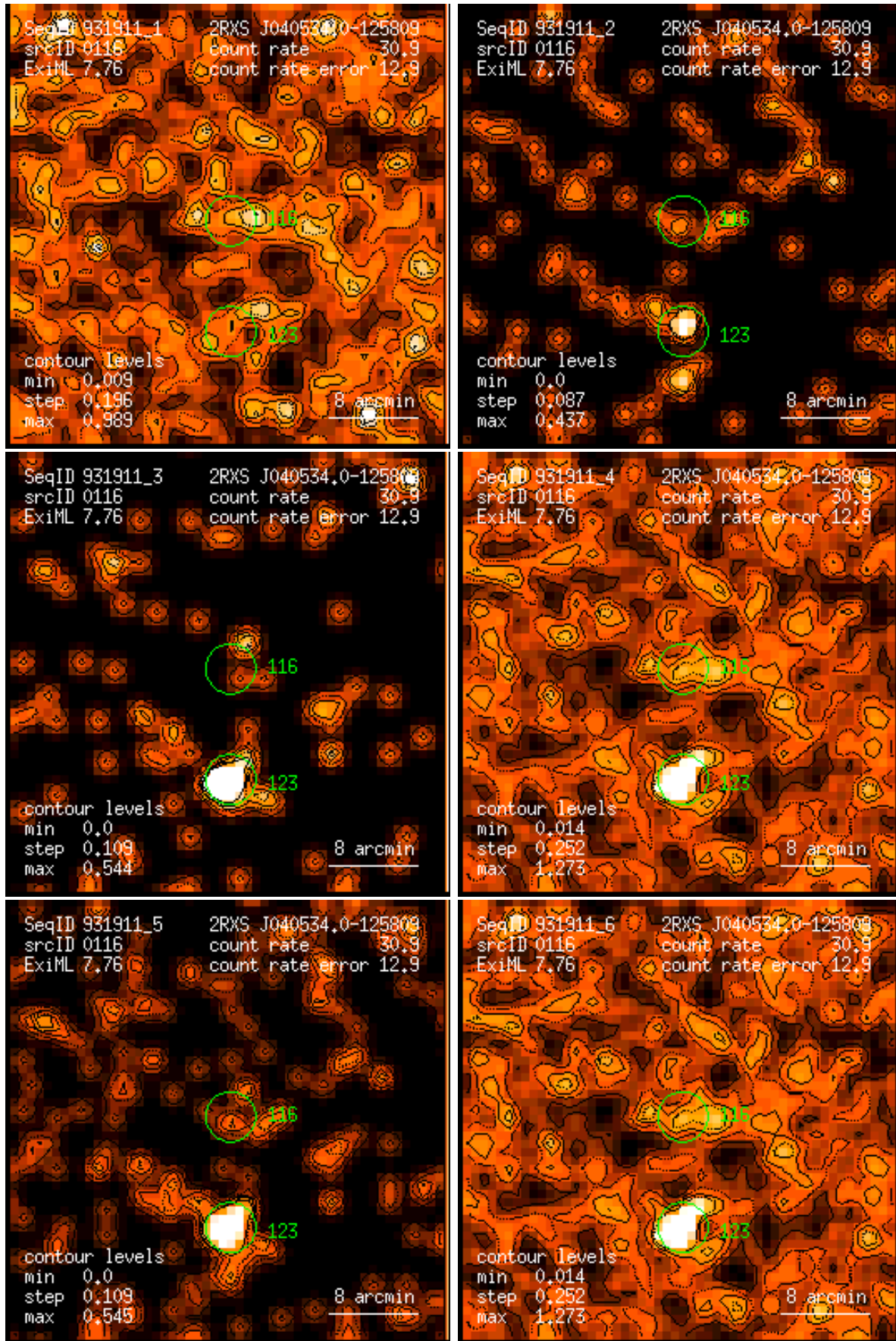
Figure 116: RASS 931911: detection 0116: band rate images, Gaussian filter: (1) PSPC channels 11 – 41, (2) 52 – 90, (3) 91 – 201, (4) 11 – 235, (5) 52 – 201, (6) 11 – 201. Broad band rates in counts/ks. Band rate contour levels in counts/ks/arcmin 2 .
