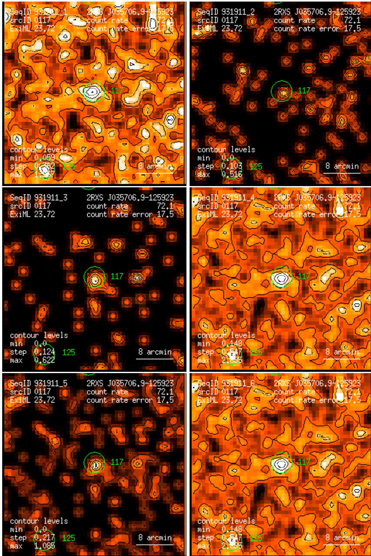
Figure 117: RASS 931911: detection 0117: band rate images, Gaussian filter: (1) PSPC channels 11 – 41, (2) 52 – 90, (3) 91 – 201, (4) 11 – 235, (5) 52 – 201, (6) 11 – 201. Broad band rates in counts/ks. Band rate contour levels in counts/ks/arcmin 2 .
