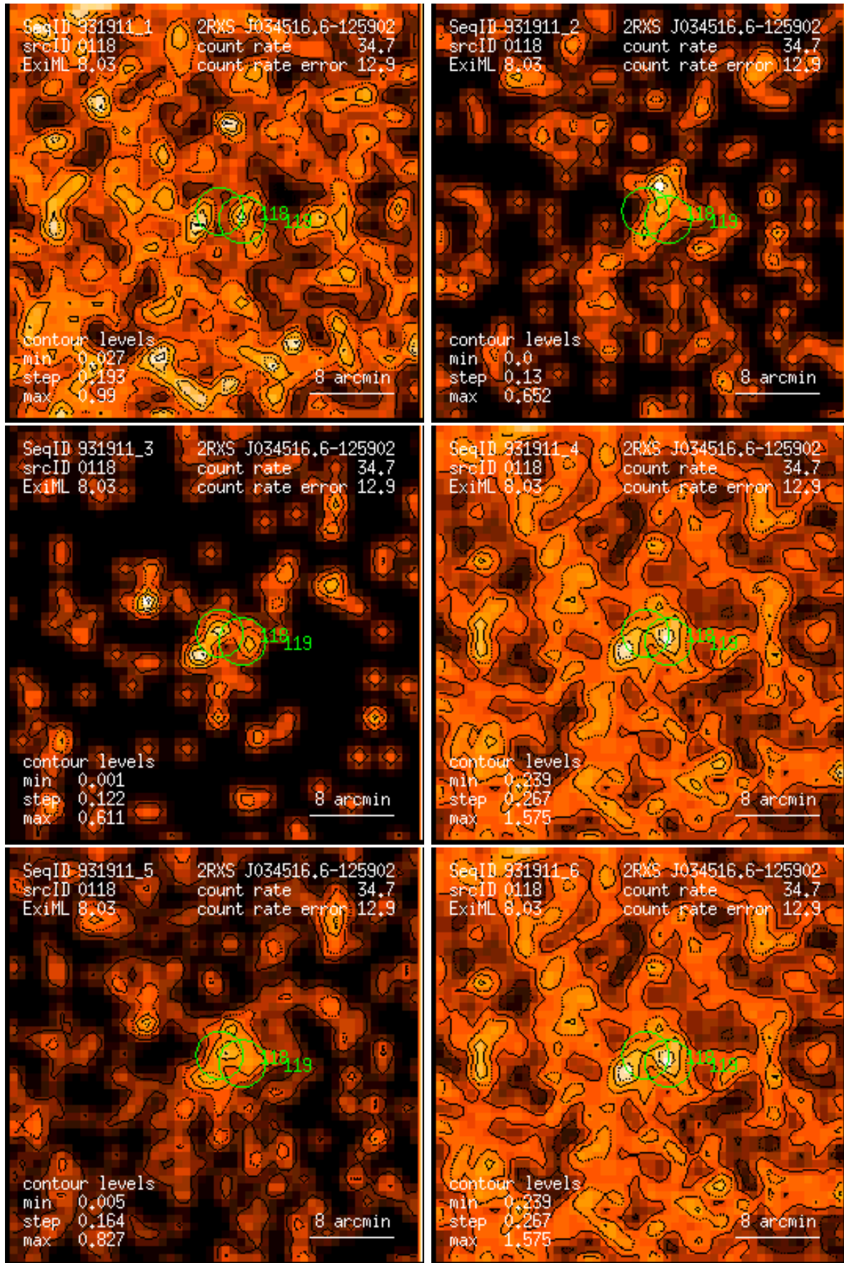
Figure 118: RASS 931911: detection 0118: band rate images, Gaussian filter: (1) PSPC channels 11 – 41, (2) 52 – 90, (3) 91 – 201, (4) 11 – 235, (5) 52 – 201, (6) 11 – 201. Broad band rates in counts/ks. Band rate contour levels in counts/ks/arcmin 2 .
