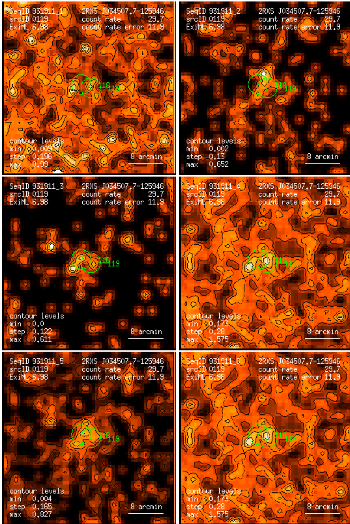
Figure 119: RASS 931911: detection 0119: band rate images, Gaussian filter: (1) PSPC channels 11 – 41, (2) 52 – 90, (3) 91 – 201, (4) 11 – 235, (5) 52 – 201, (6) 11 – 201. Broad band rates in counts/ks. Band rate contour levels in counts/ks/arcmin 2 .
