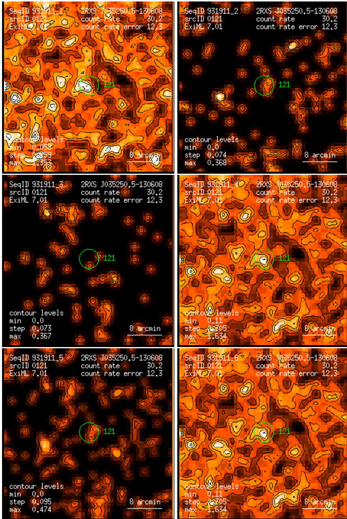
Figure 121: RASS 931911: detection 0121: band rate images, Gaussian filter: (1) PSPC channels 11 – 41, (2) 52 – 90, (3) 91 – 201, (4) 11 – 235, (5) 52 – 201, (6) 11 – 201. Broad band rates in counts/ks. Band rate contour levels in counts/ks/arcmin 2 .
