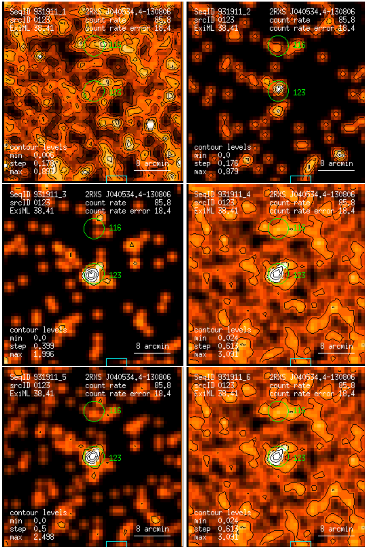
Figure 123: RASS 931911: detection 0123: band rate images, Gaussian filter: (1) PSPC channels 11 – 41, (2) 52 – 90, (3) 91 – 201, (4) 11 – 235, (5) 52 – 201, (6) 11 – 201. Broad band rates in counts/ks. Band rate contour levels in counts/ks/arcmin 2 .
