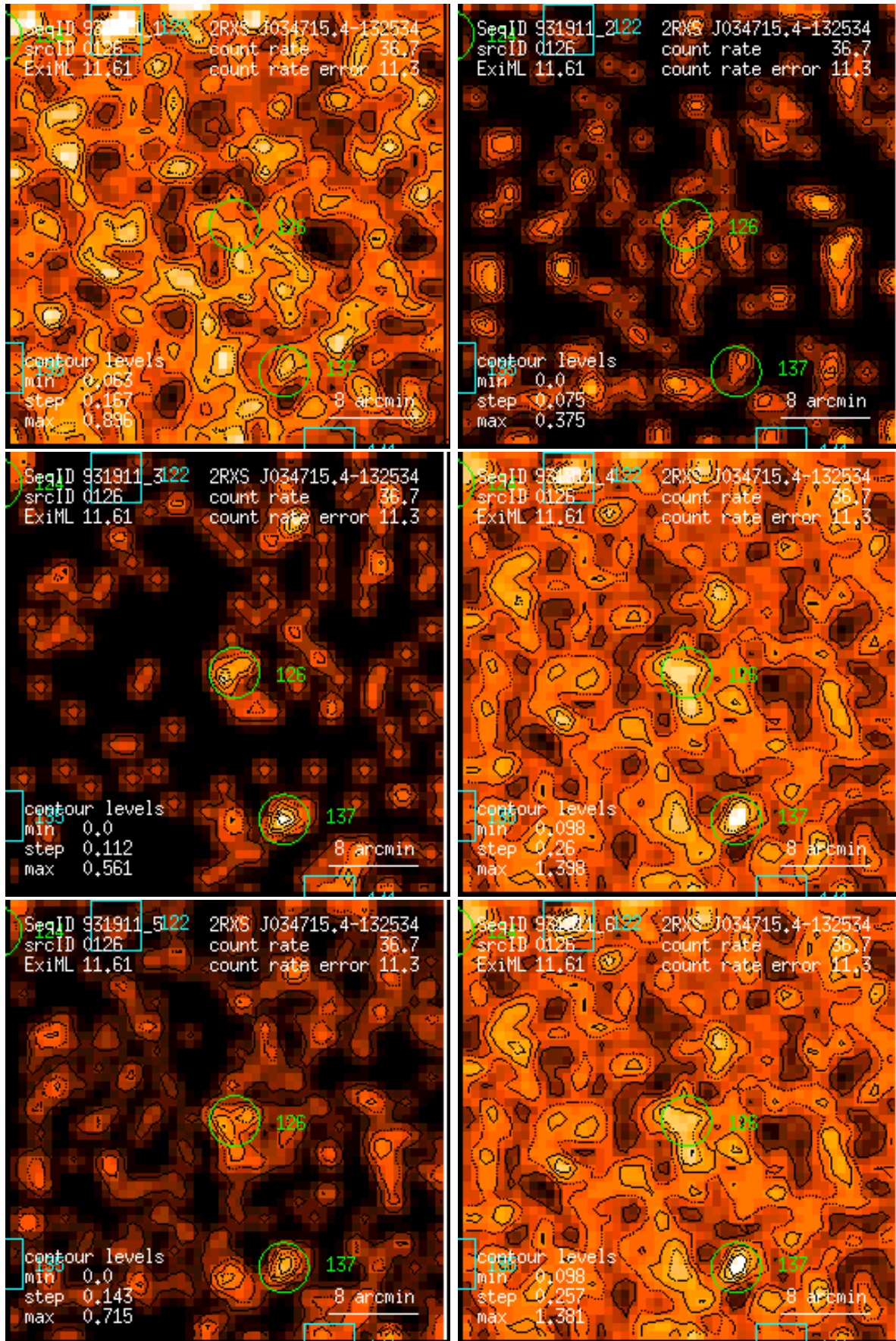
Figure 126: RASS 931911: detection 0126: band rate images, Gaussian filter: (1) PSPC channels 11 – 41, (2) 52 – 90, (3) 91 – 201, (4) 11 – 235, (5) 52 – 201, (6) 11 – 201. Broad band rates in counts/ks. Band rate contour levels in counts/ks/arcmin 2 .
