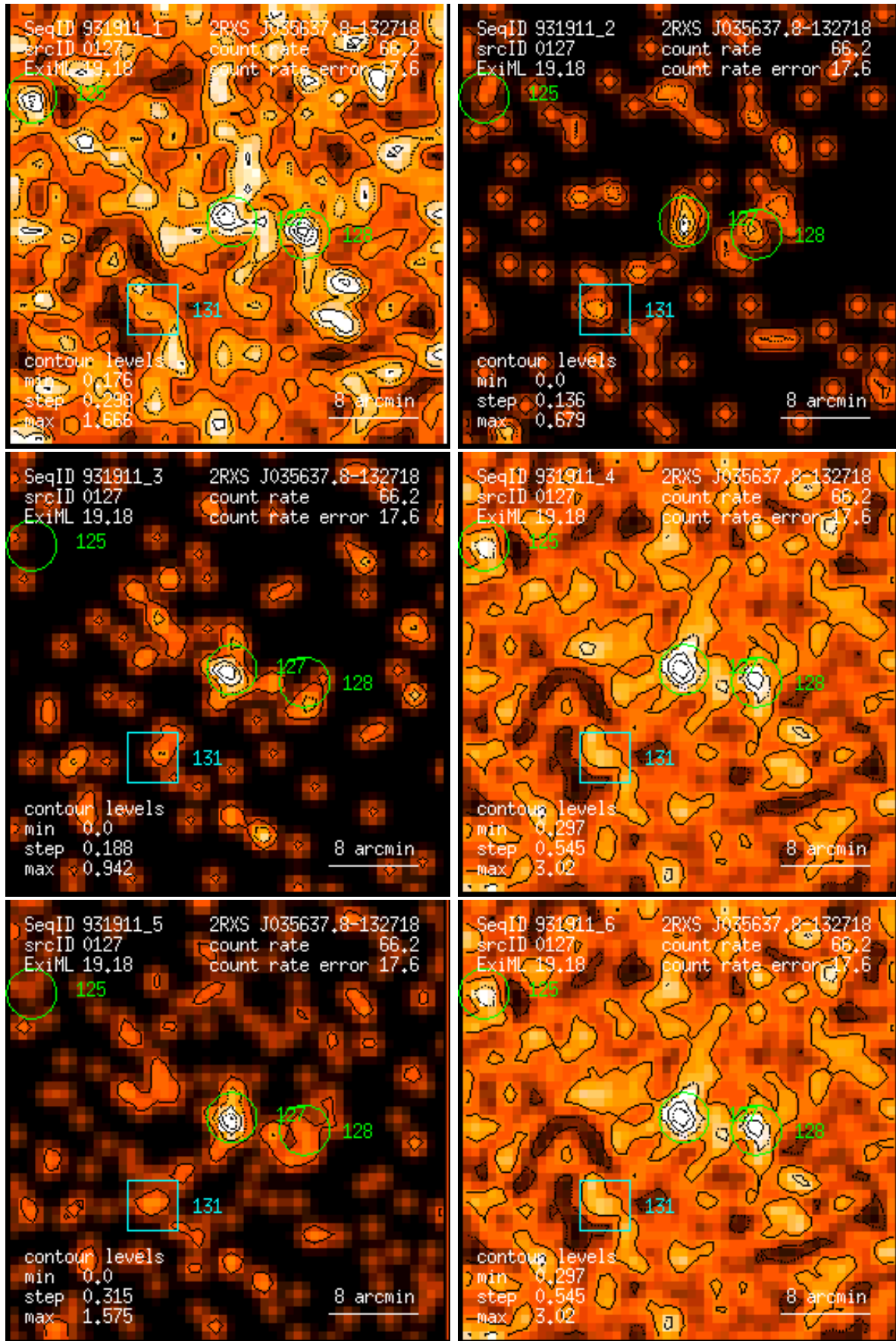
Figure 127: RASS 931911: detection 0127: band rate images, Gaussian filter: (1) PSPC channels 11 – 41, (2) 52 – 90, (3) 91 – 201, (4) 11 – 235, (5) 52 – 201, (6) 11 – 201. Broad band rates in counts/ks. Band rate contour levels in counts/ks/arcmin 2 .
