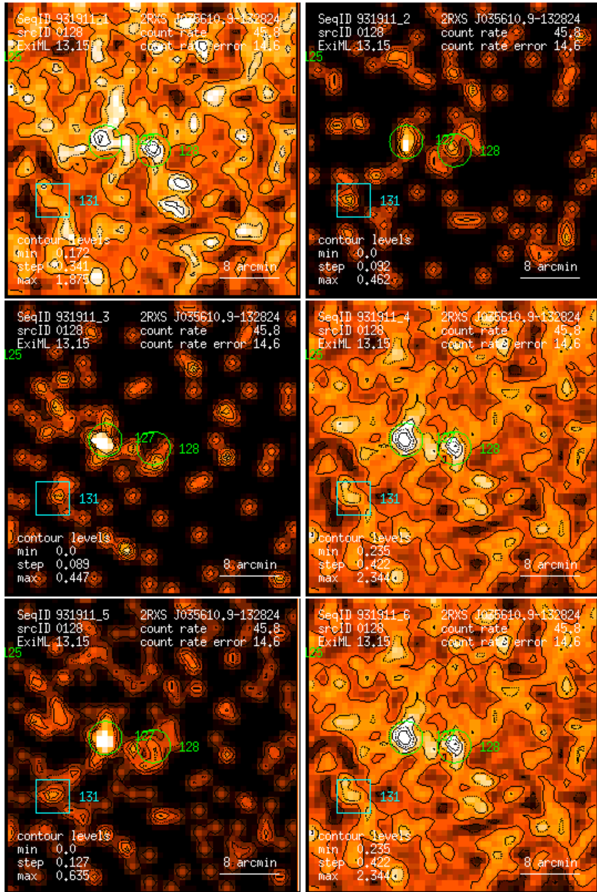
Figure 128: RASS 931911: detection 0128: band rate images, Gaussian filter: (1) PSPC channels 11 – 41, (2) 52 – 90, (3) 91 – 201, (4) 11 – 235, (5) 52 – 201, (6) 11 – 201. Broad band rates in counts/ks. Band rate contour levels in counts/ks/arcmin 2 .
