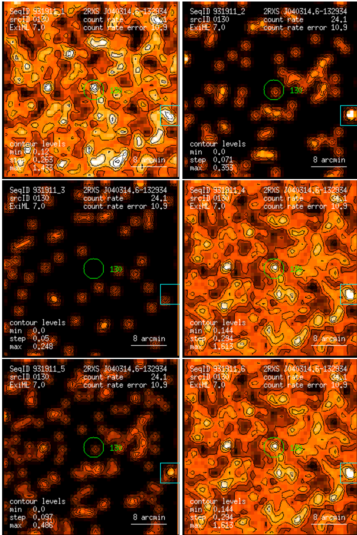
Figure 130: RASS 931911: detection 0130: band rate images, Gaussian filter: (1) PSPC channels 11 – 41, (2) 52 – 90, (3) 91 – 201, (4) 11 – 235, (5) 52 – 201, (6) 11 – 201. Broad band rates in counts/ks. Band rate contour levels in counts/ks/arcmin 2 .
