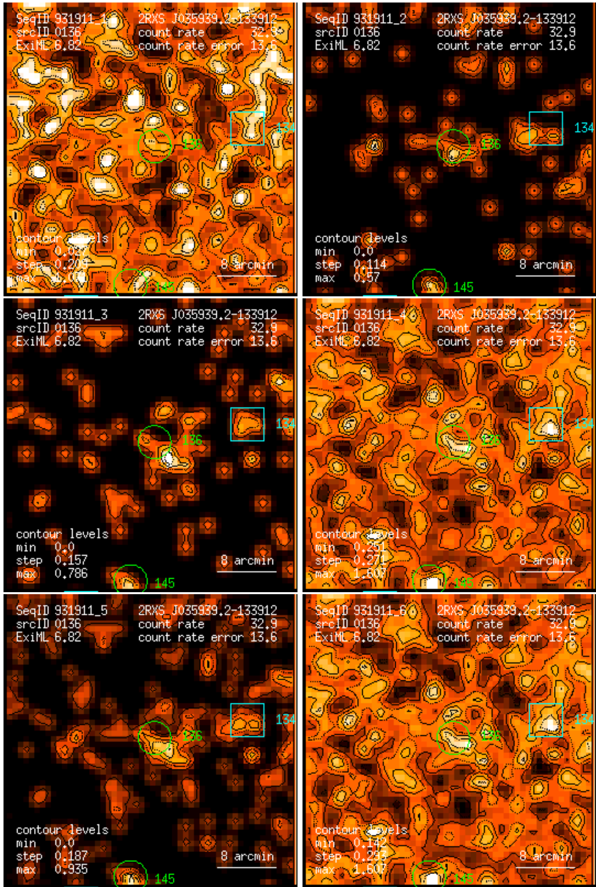
Figure 136: RASS 931911: detection 0136: band rate images, Gaussian filter: (1) PSPC channels 11 – 41, (2) 52 – 90, (3) 91 – 201, (4) 11 – 235, (5) 52 – 201, (6) 11 – 201. Broad band rates in counts/ks. Band rate contour levels in counts/ks/arcmin 2 .
