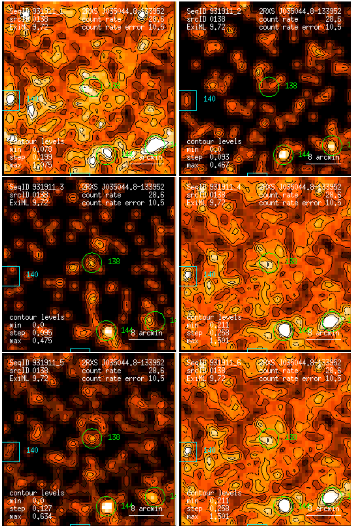
Figure 138: RASS 931911: detection 0138: band rate images, Gaussian filter: (1) PSPC channels 11 – 41, (2) 52 – 90, (3) 91 – 201, (4) 11 – 235, (5) 52 – 201, (6) 11 – 201. Broad band rates in counts/ks. Band rate contour levels in counts/ks/arcmin 2 .
