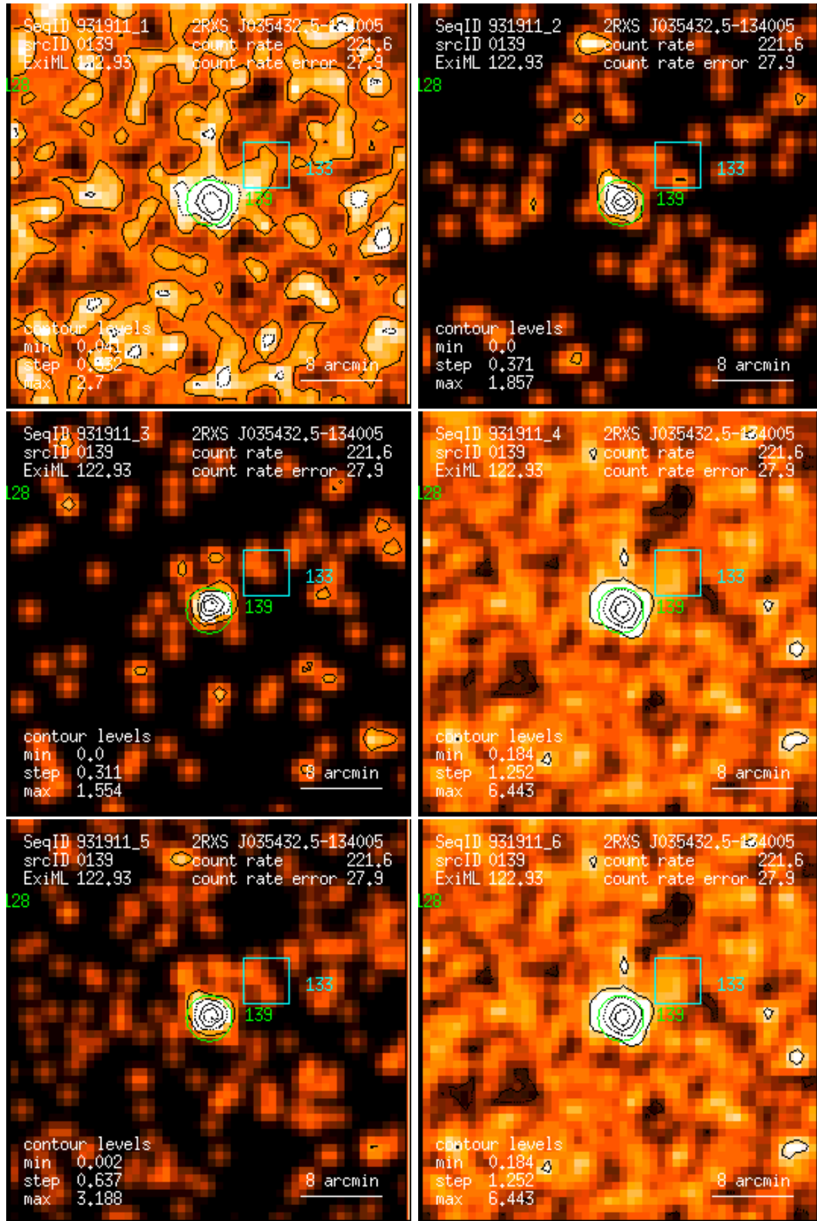
Figure 139: RASS 931911: detection 0139: band rate images, Gaussian filter: (1) PSPC channels 11 – 41, (2) 52 – 90, (3) 91 – 201, (4) 11 – 235, (5) 52 – 201, (6) 11 – 201. Broad band rates in counts/ks. Band rate contour levels in counts/ks/arcmin 2 .
