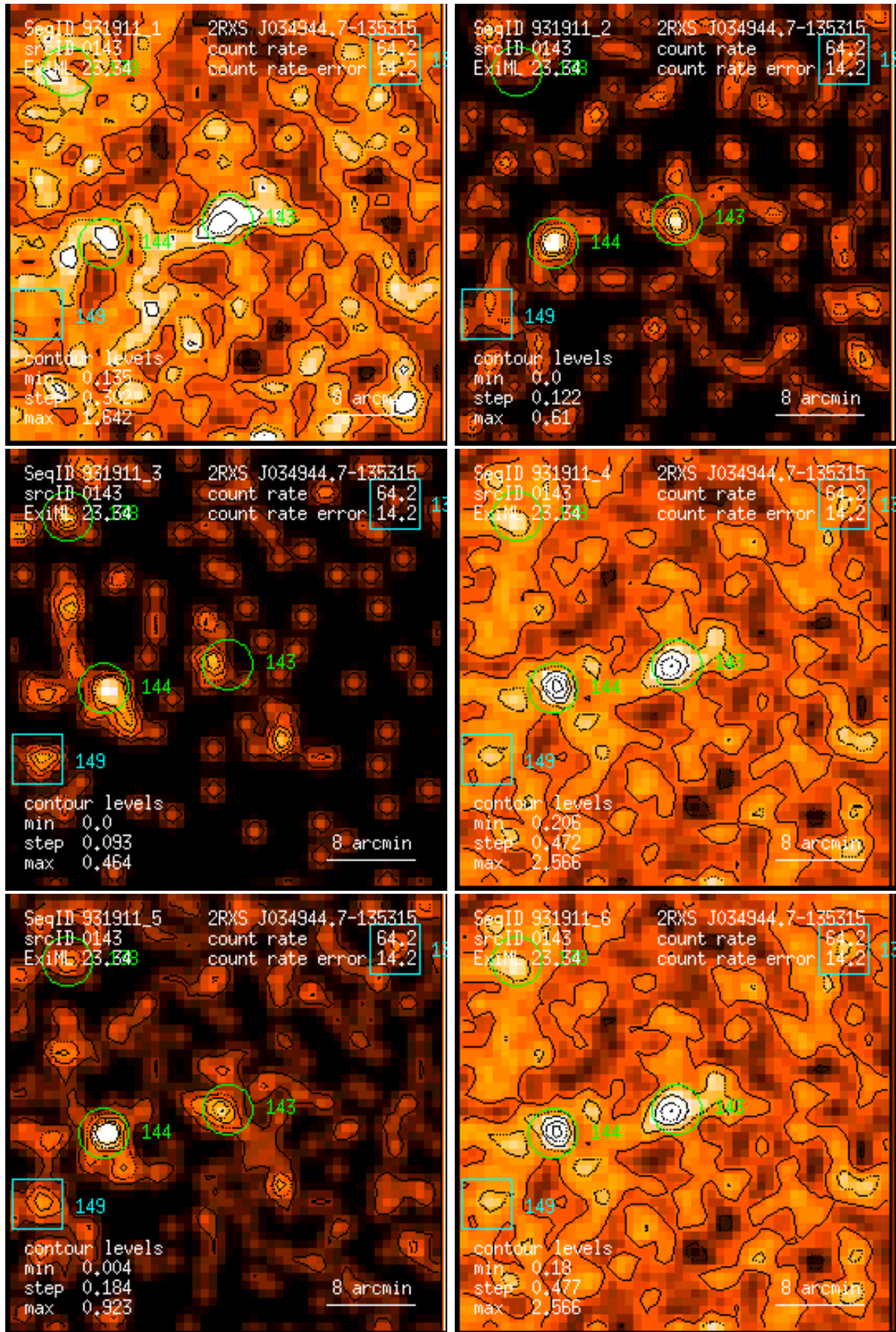
Figure 143: RASS 931911: detection 0143: band rate images, Gaussian filter: (1) PSPC channels 11 – 41, (2) 52 – 90, (3) 91 – 201, (4) 11 – 235, (5) 52 – 201, (6) 11 – 201. Broad band rates in counts/ks. Band rate contour levels in counts/ks/arcmin 2 .
