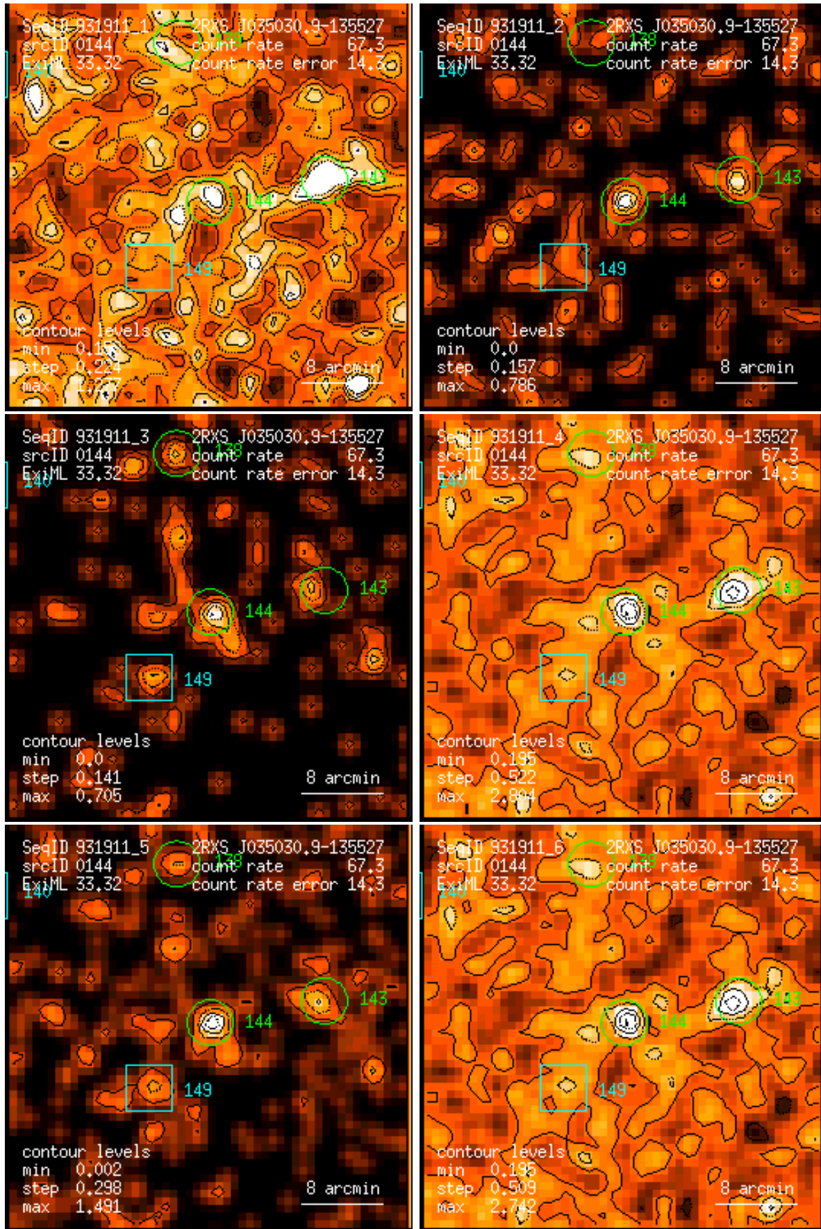
Figure 144: RASS 931911: detection 0144: band rate images, Gaussian filter: (1) PSPC channels 11 – 41, (2) 52 – 90, (3) 91 – 201, (4) 11 – 235, (5) 52 – 201, (6) 11 – 201. Broad band rates in counts/ks. Band rate contour levels in counts/ks/arcmin 2 .
