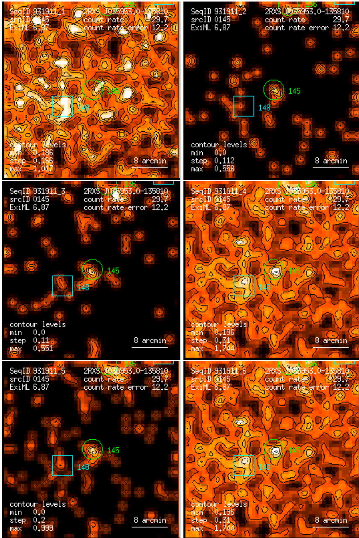
Figure 145: RASS 931911: detection 0145: band rate images, Gaussian filter: (1) PSPC channels 11 – 41, (2) 52 – 90, (3) 91 – 201, (4) 11 – 235, (5) 52 – 201, (6) 11 – 201. Broad band rates in counts/ks. Band rate contour levels in counts/ks/arcmin 2 .
