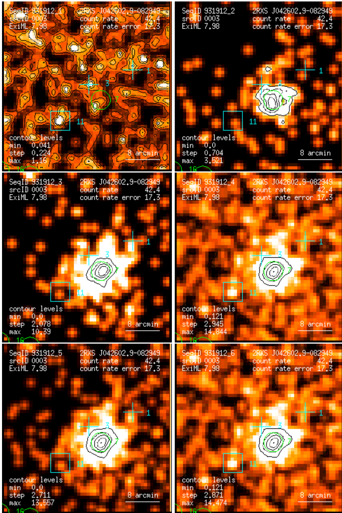
Figure 3: RASS 931912: detection 0003: band rate images, Gaussian filter: (1) PSPC channels 11 – 41, (2) 52 – 90, (3) 91 – 201, (4) 11 – 235, (5) 52 – 201, (6) 11 – 201. Broad band rates in counts/ks. Band rate contour levels in counts/ks/arcmin 2 .
