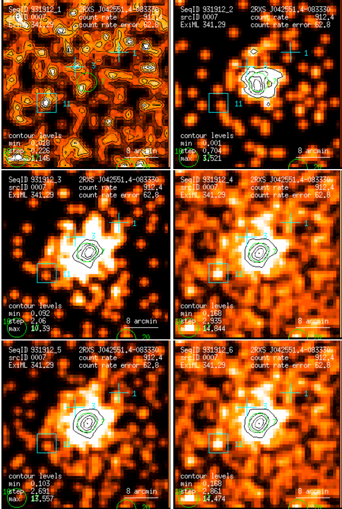
Figure 7: RASS 931912: detection 0007: band rate images, Gaussian filter: (1) PSPC channels 11 – 41, (2) 52 – 90, (3) 91 – 201, (4) 11 – 235, (5) 52 – 201, (6) 11 – 201. Broad band rates in counts/ks. Band rate contour levels in counts/ks/arcmin 2 .
