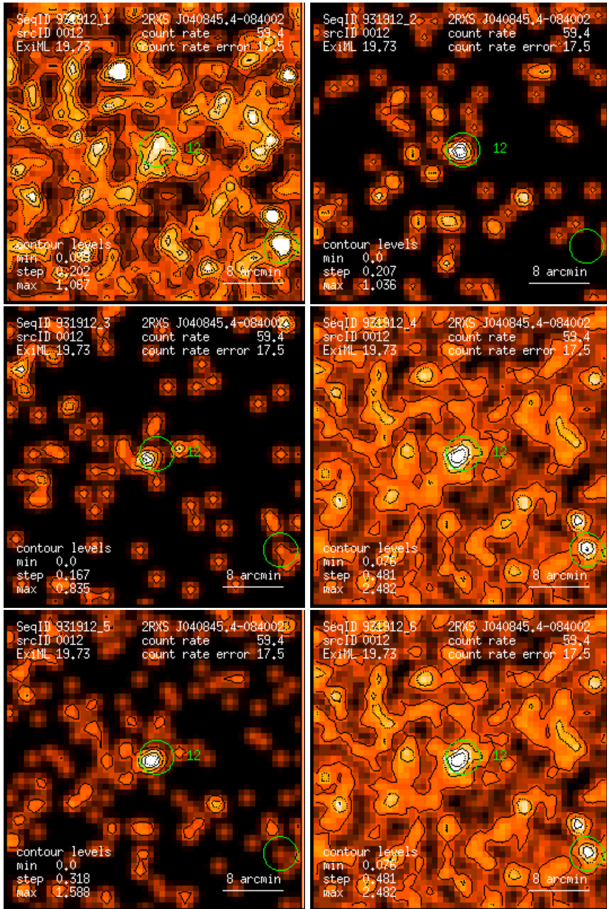
Figure 12: RASS 931912: detection 0012: band rate images, Gaussian filter: (1) PSPC channels 11 – 41, (2) 52 – 90, (3) 91 – 201, (4) 11 – 235, (5) 52 – 201, (6) 11 – 201. Broad band rates in counts/ks. Band rate contour levels in counts/ks/arcmin 2 .
