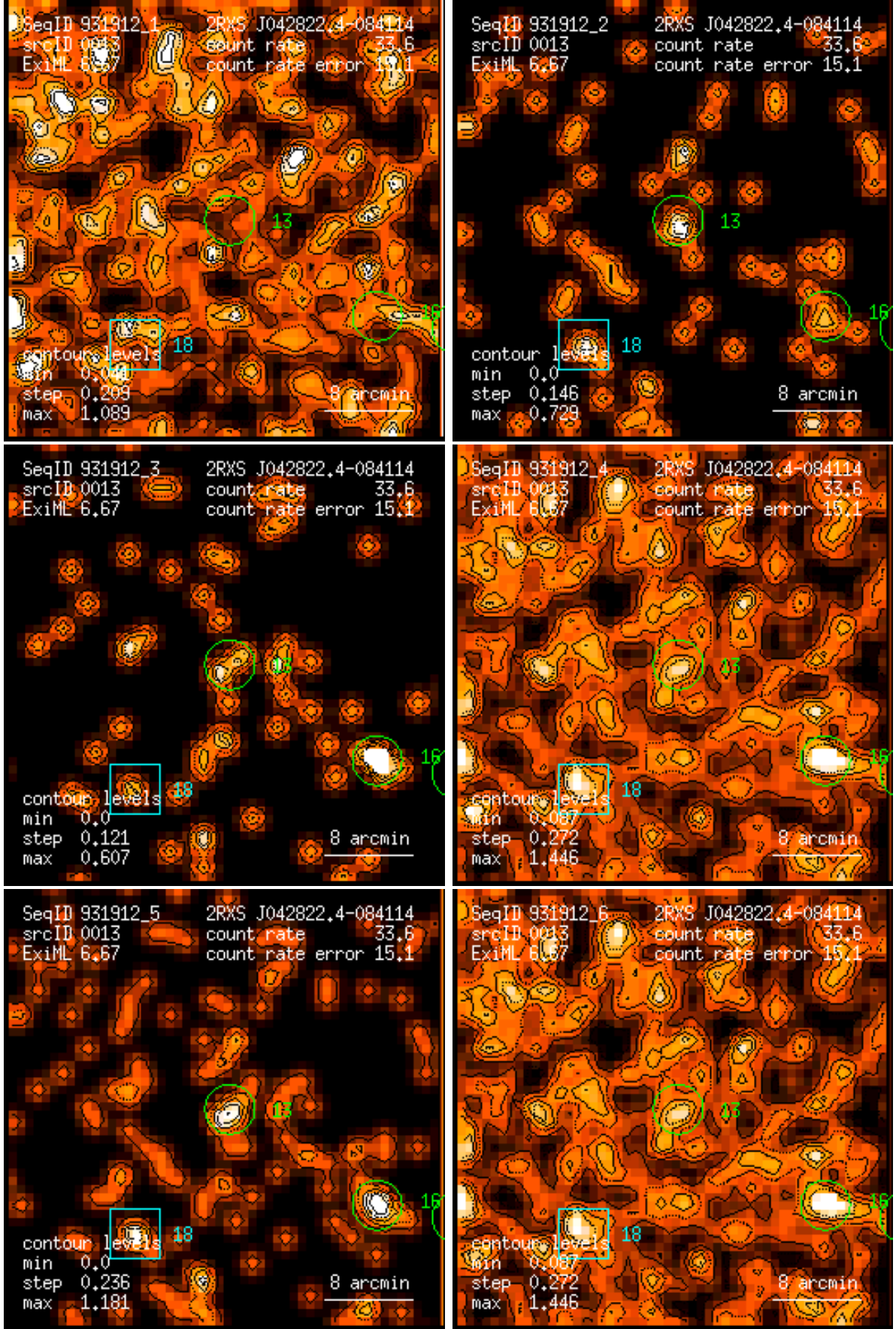
Figure 13: RASS 931912: detection 0013: band rate images, Gaussian filter: (1) PSPC channels 11 – 41, (2) 52 – 90, (3) 91 – 201, (4) 11 – 235, (5) 52 – 201, (6) 11 – 201. Broad band rates in counts/ks. Band rate contour levels in counts/ks/arcmin 2 .
