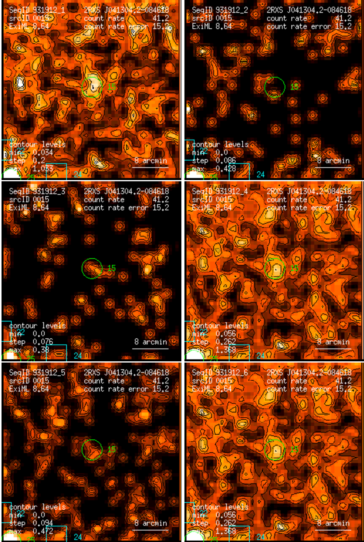
Figure 15: RASS 931912: detection 0015: band rate images, Gaussian filter: (1) PSPC channels 11 – 41, (2) 52 – 90, (3) 91 – 201, (4) 11 – 235, (5) 52 – 201, (6) 11 – 201. Broad band rates in counts/ks. Band rate contour levels in counts/ks/arcmin 2 .
