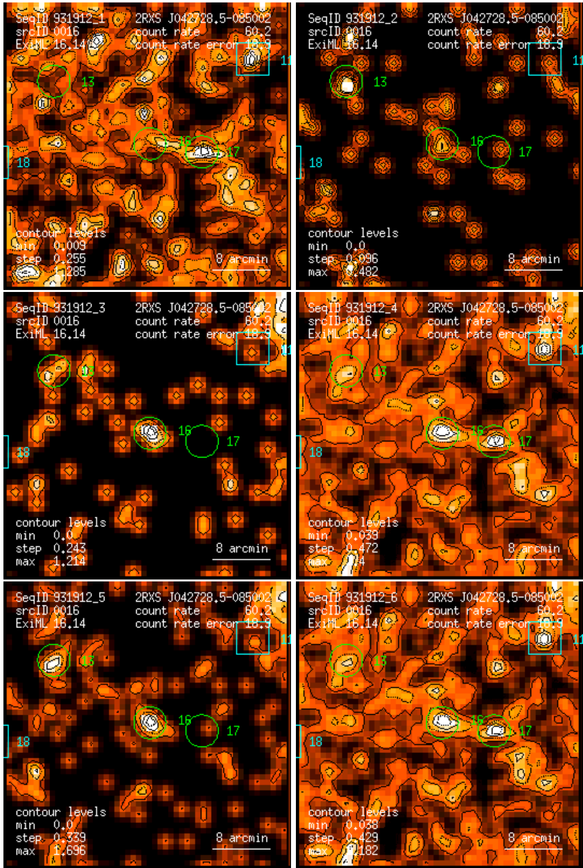
Figure 16: RASS 931912: detection 0016: band rate images, Gaussian filter: (1) PSPC channels 11 – 41, (2) 52 – 90, (3) 91 – 201, (4) 11 – 235, (5) 52 – 201, (6) 11 – 201. Broad band rates in counts/ks. Band rate contour levels in counts/ks/arcmin 2 .
