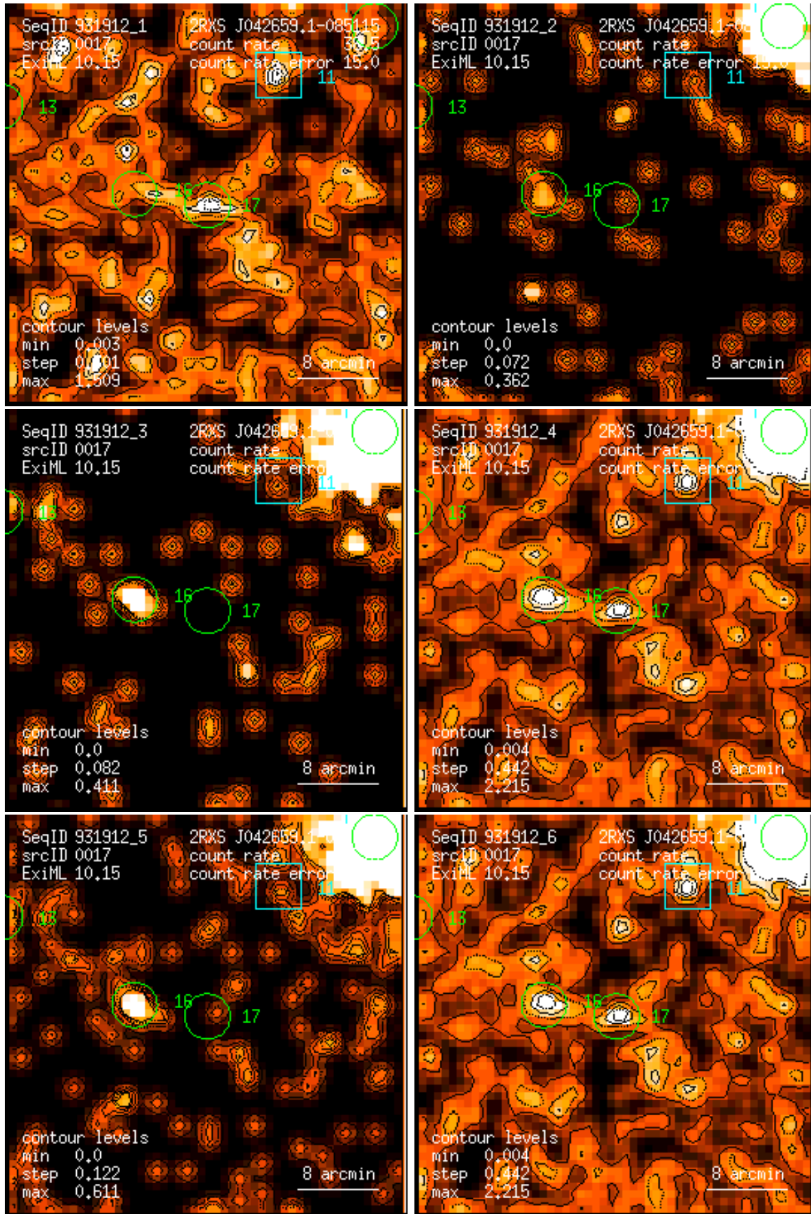
Figure 17: RASS 931912: detection 0017: band rate images, Gaussian filter: (1) PSPC channels 11 – 41, (2) 52 – 90, (3) 91 – 201, (4) 11 – 235, (5) 52 – 201, (6) 11 – 201. Broad band rates in counts/ks. Band rate contour levels in counts/ks/arcmin 2 .
