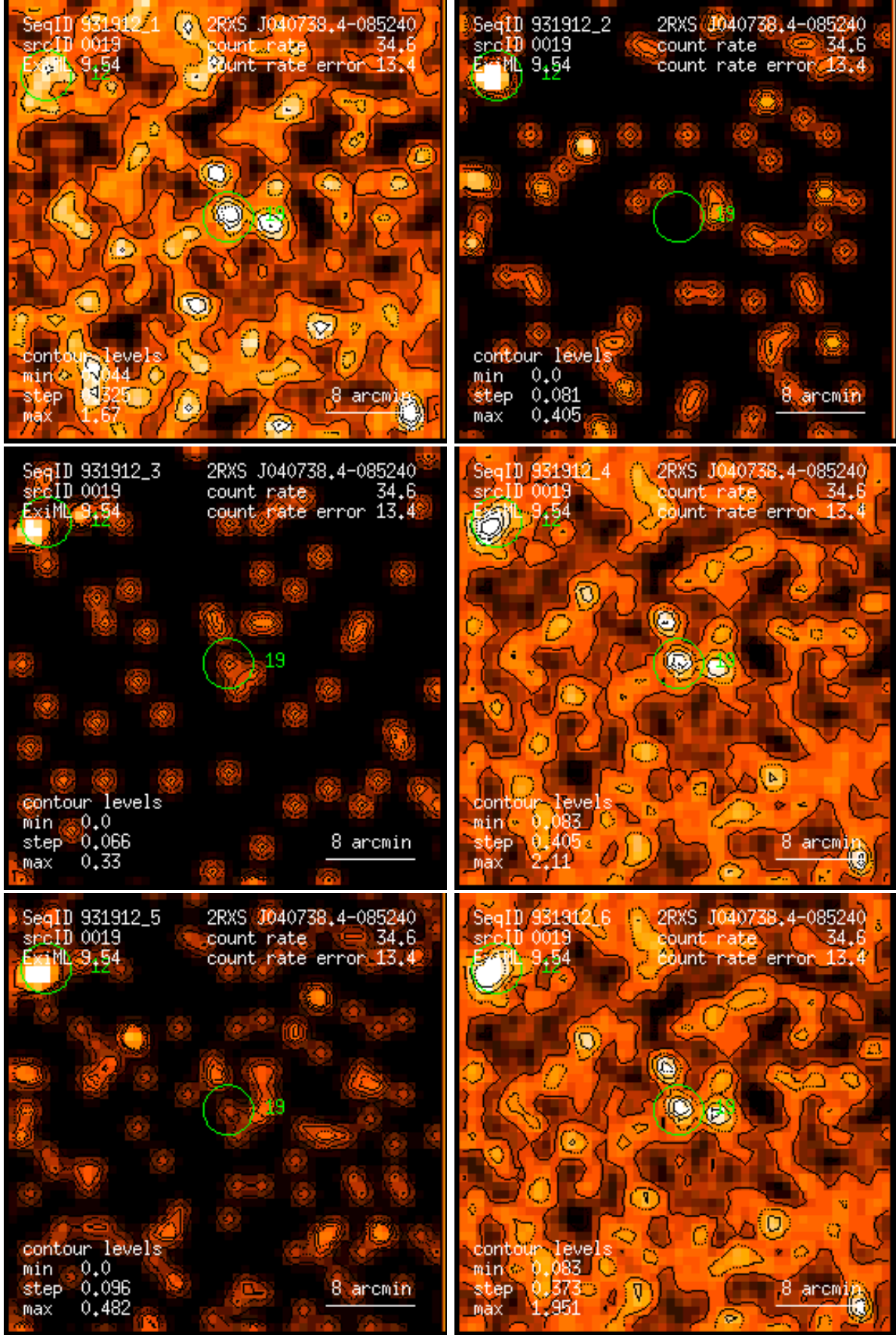
Figure 19: RASS 931912: detection 0019: band rate images, Gaussian filter: (1) PSPC channels 11 – 41, (2) 52 – 90, (3) 91 – 201, (4) 11 – 235, (5) 52 – 201, (6) 11 – 201. Broad band rates in counts/ks. Band rate contour levels in counts/ks/arcmin 2 .
