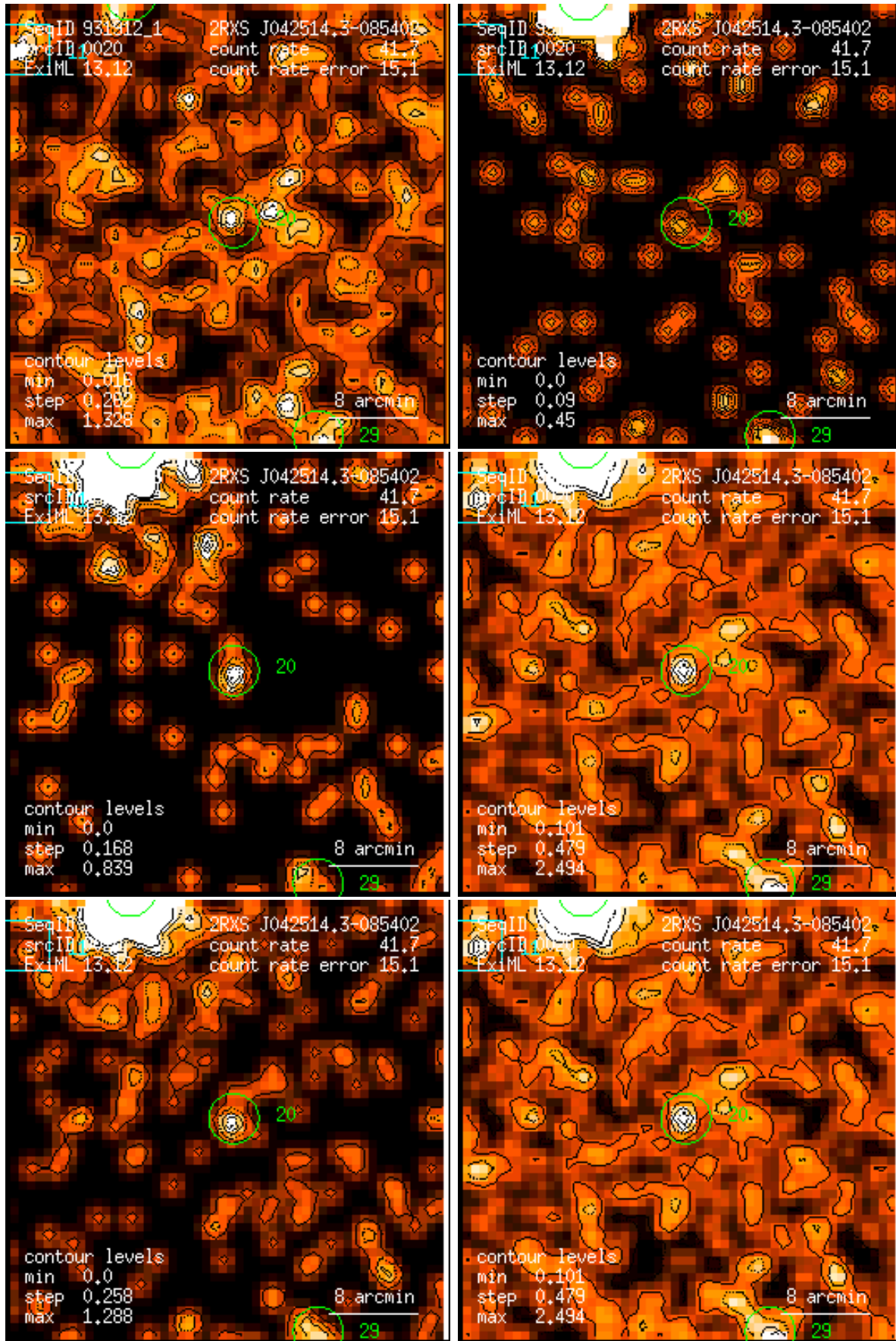
Figure 20: RASS 931912: detection 0020: band rate images, Gaussian filter: (1) PSPC channels 11 – 41, (2) 52 – 90, (3) 91 – 201, (4) 11 – 235, (5) 52 – 201, (6) 11 – 201. Broad band rates in counts/ks. Band rate contour levels in counts/ks/arcmin 2 .
