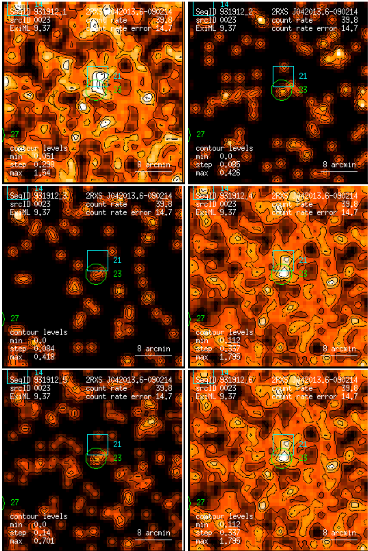
Figure 23: RASS 931912: detection 0023: band rate images, Gaussian filter: (1) PSPC channels 11 – 41, (2) 52 – 90, (3) 91 – 201, (4) 11 – 235, (5) 52 – 201, (6) 11 – 201. Broad band rates in counts/ks. Band rate contour levels in counts/ks/arcmin 2 .
