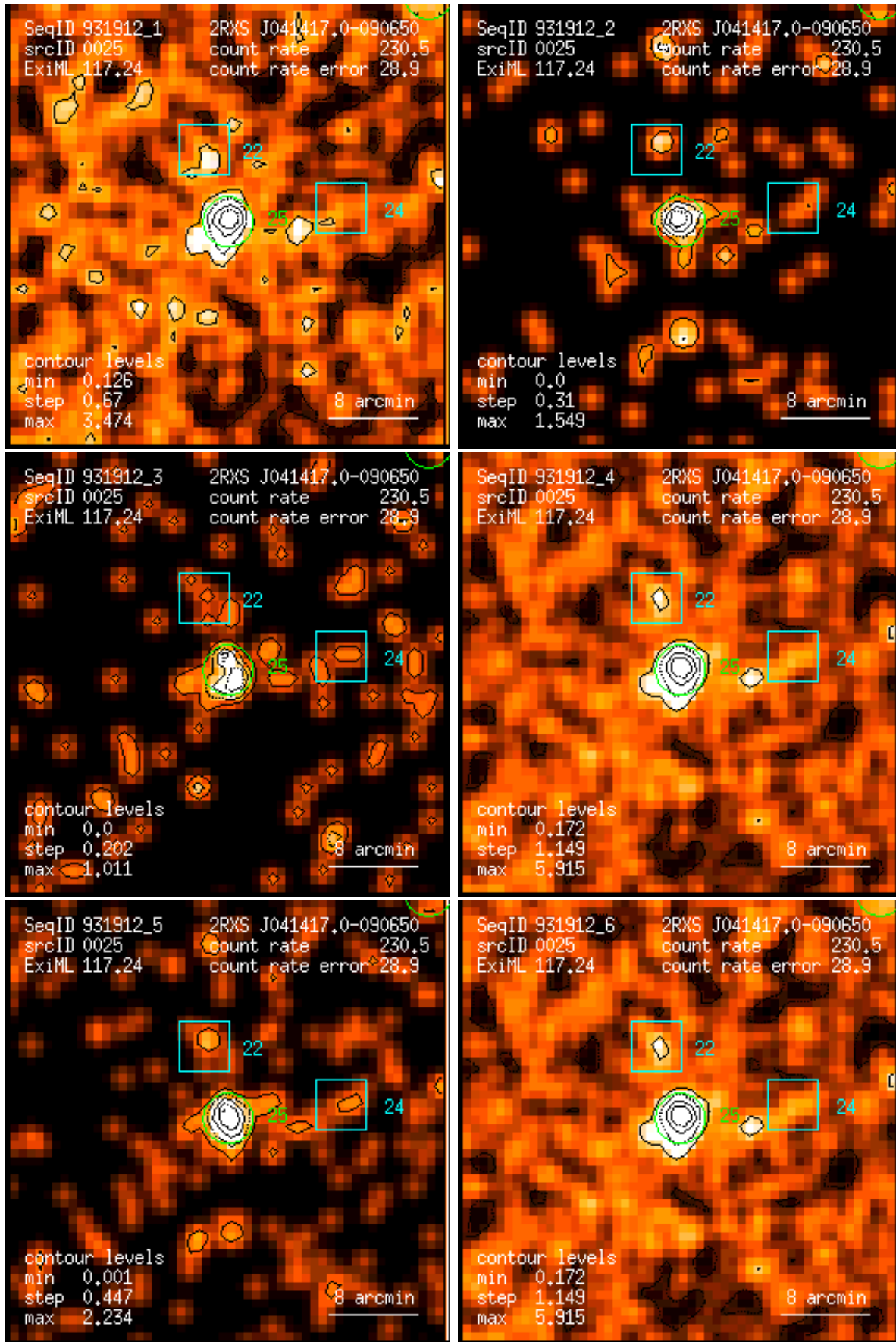
Figure 25: RASS 931912: detection 0025: band rate images, Gaussian filter: (1) PSPC channels 11 – 41, (2) 52 – 90, (3) 91 – 201, (4) 11 – 235, (5) 52 – 201, (6) 11 – 201. Broad band rates in counts/ks. Band rate contour levels in counts/ks/arcmin 2 .
