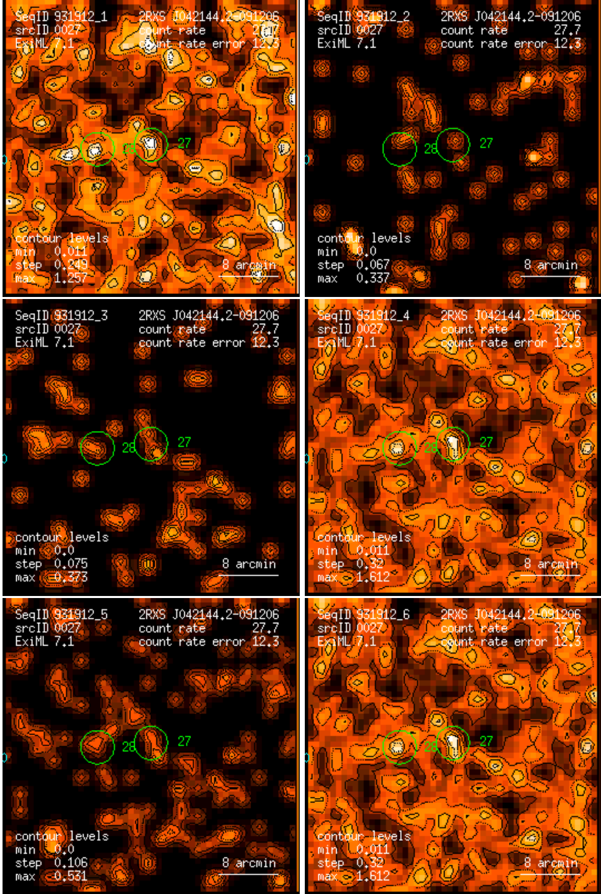
Figure 27: RASS 931912: detection 0027: band rate images, Gaussian filter: (1) PSPC channels 11 – 41, (2) 52 – 90, (3) 91 – 201, (4) 11 – 235, (5) 52 – 201, (6) 11 – 201. Broad band rates in counts/ks. Band rate contour levels in counts/ks/arcmin 2 .
