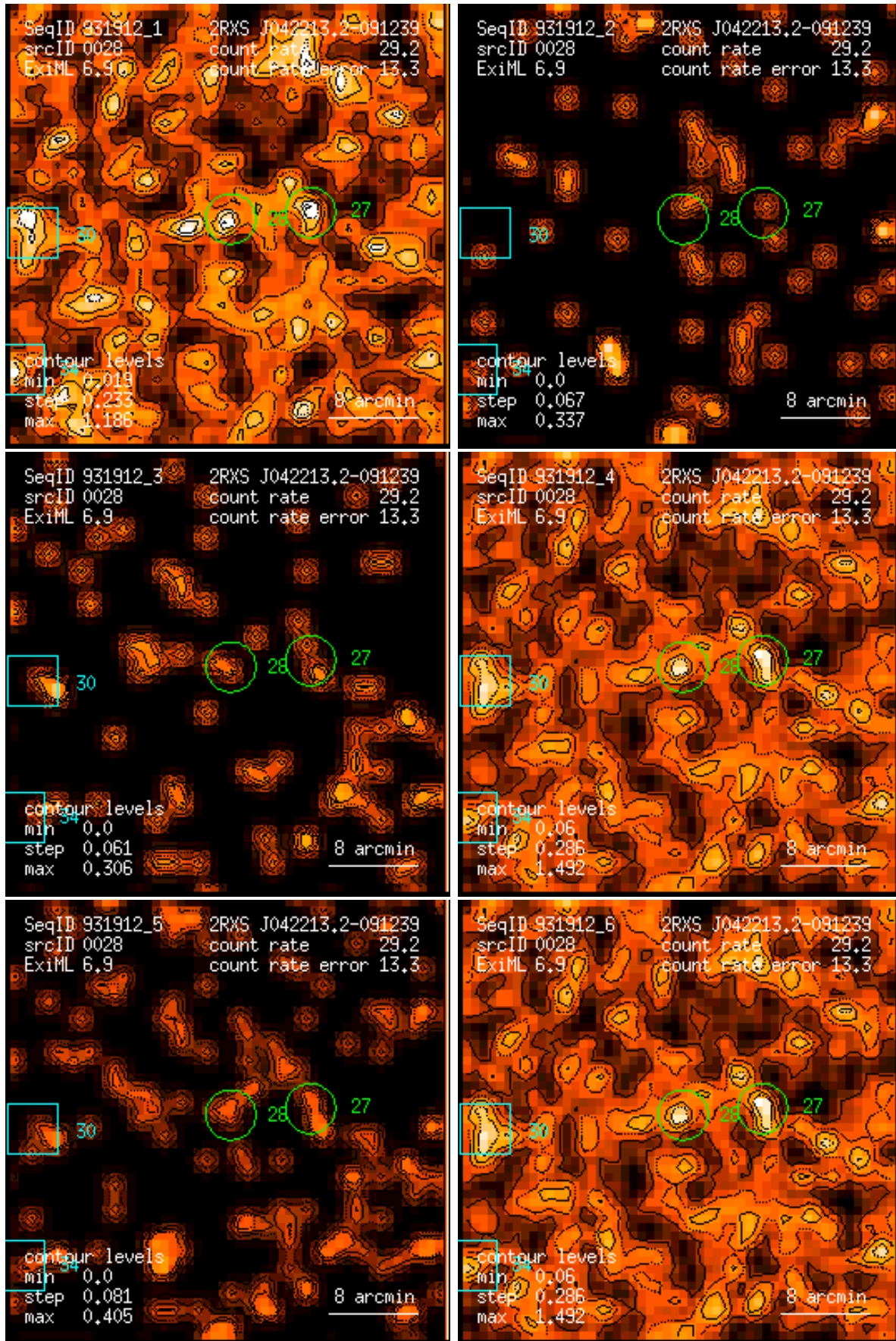
Figure 28: RASS 931912: detection 0028: band rate images, Gaussian filter: (1) PSPC channels 11 – 41, (2) 52 – 90, (3) 91 – 201, (4) 11 – 235, (5) 52 – 201, (6) 11 – 201. Broad band rates in counts/ks. Band rate contour levels in counts/ks/arcmin 2 .
