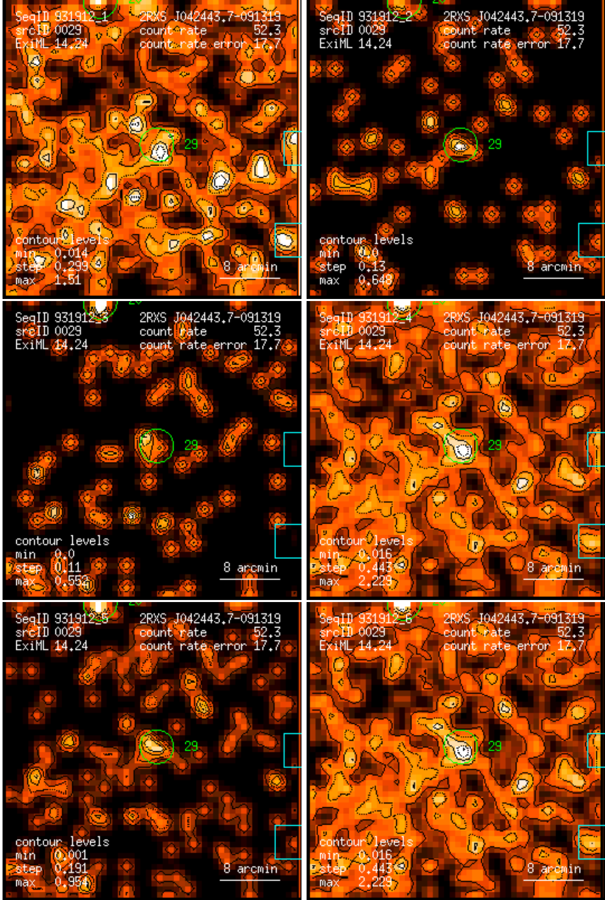
Figure 29: RASS 931912: detection 0029: band rate images, Gaussian filter: (1) PSPC channels 11 – 41, (2) 52 – 90, (3) 91 – 201, (4) 11 – 235, (5) 52 – 201, (6) 11 – 201. Broad band rates in counts/ks. Band rate contour levels in counts/ks/arcmin 2 .
