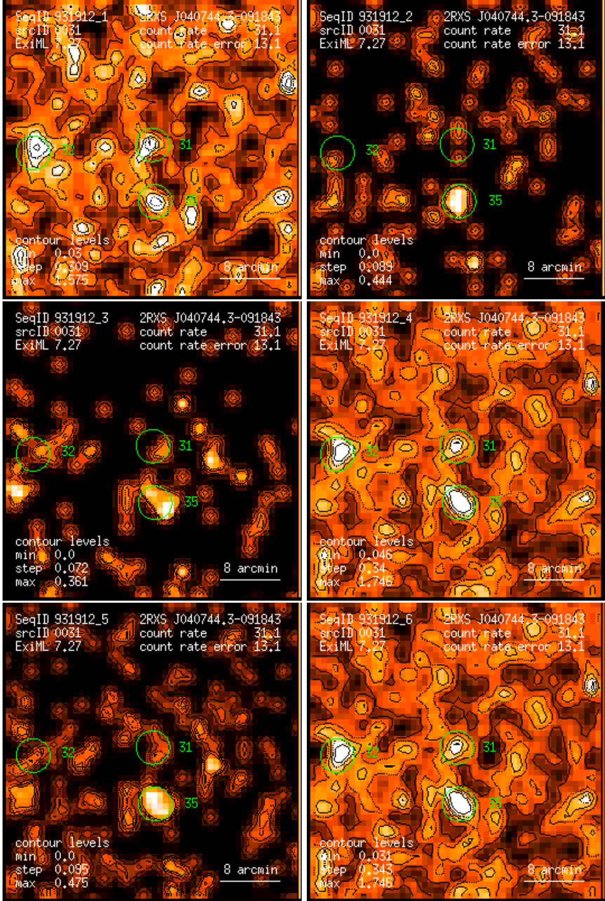
Figure 31: RASS 931912: detection 0031: band rate images, Gaussian filter: (1) PSPC channels 11 – 41, (2) 52 – 90, (3) 91 – 201, (4) 11 – 235, (5) 52 – 201, (6) 11 – 201. Broad band rates in counts/ks. Band rate contour levels in counts/ks/arcmin 2 .
