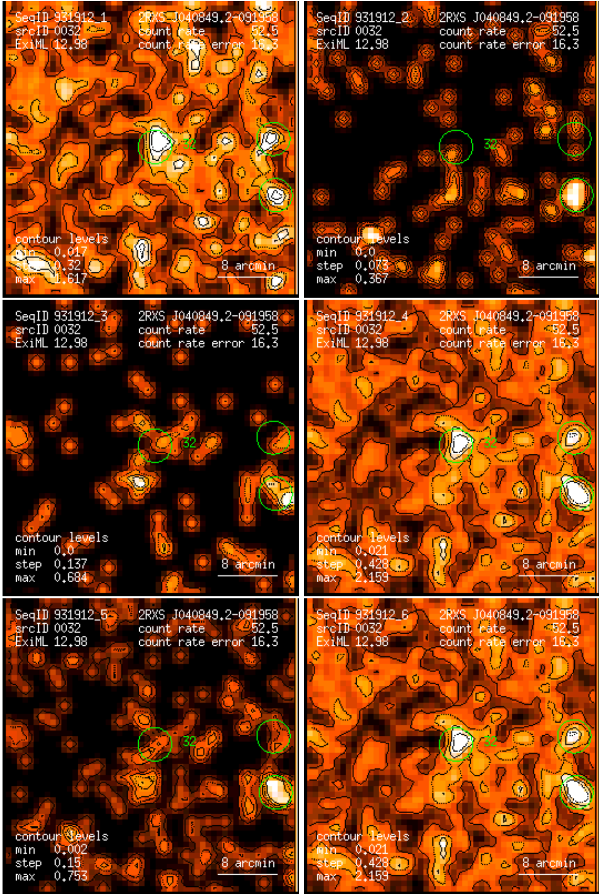
Figure 32: RASS 931912: detection 0032: band rate images, Gaussian filter: (1) PSPC channels 11 – 41, (2) 52 – 90, (3) 91 – 201, (4) 11 – 235, (5) 52 – 201, (6) 11 – 201. Broad band rates in counts/ks. Band rate contour levels in counts/ks/arcmin 2 .
