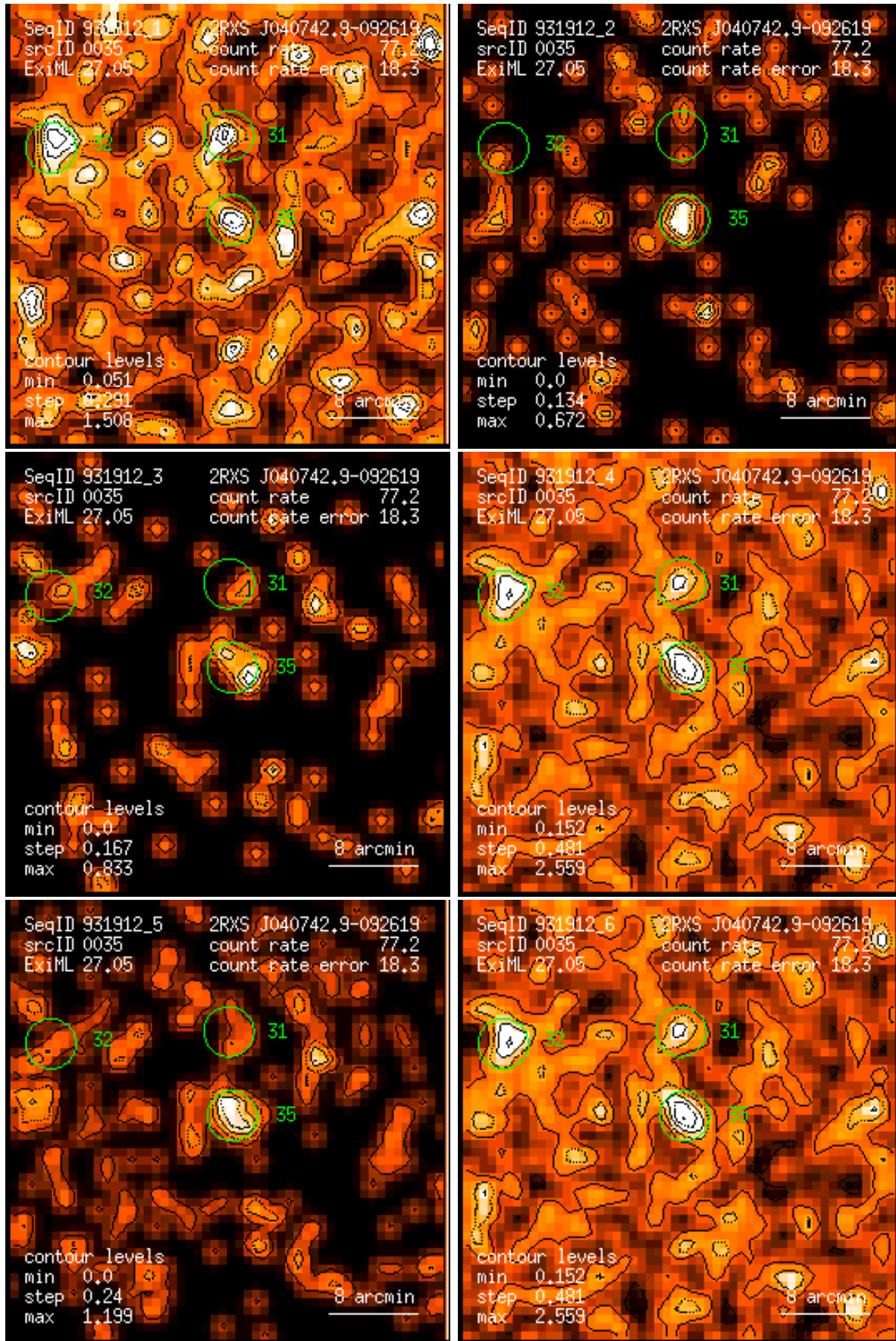
Figure 35: RASS 931912: detection 0035: band rate images, Gaussian filter: (1) PSPC channels 11 – 41, (2) 52 – 90, (3) 91 – 201, (4) 11 – 235, (5) 52 – 201, (6) 11 – 201. Broad band rates in counts/ks. Band rate contour levels in counts/ks/arcmin 2 .
