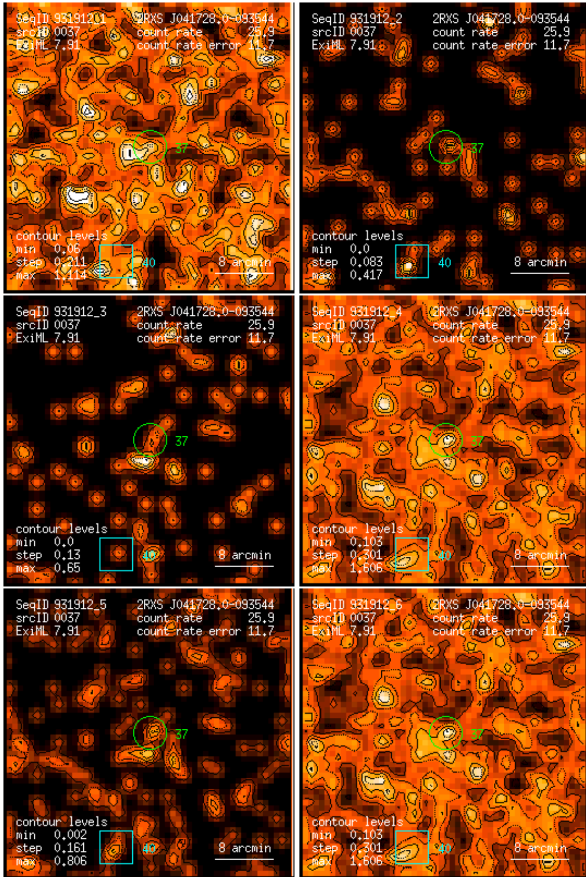
Figure 37: RASS 931912: detection 0037: band rate images, Gaussian filter: (1) PSPC channels 11 – 41, (2) 52 – 90, (3) 91 – 201, (4) 11 – 235, (5) 52 – 201, (6) 11 – 201. Broad band rates in counts/ks. Band rate contour levels in counts/ks/arcmin 2 .
