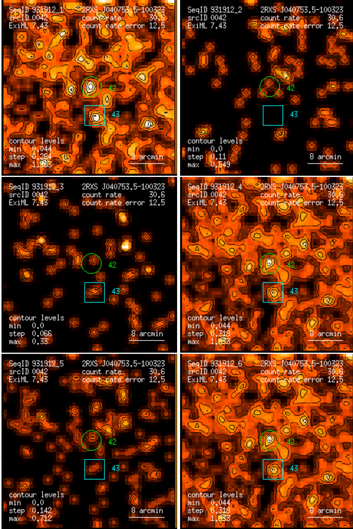
Figure 42: RASS 931912: detection 0042: band rate images, Gaussian filter: (1) PSPC channels 11 – 41, (2) 52 – 90, (3) 91 – 201, (4) 11 – 235, (5) 52 – 201, (6) 11 – 201. Broad band rates in counts/ks. Band rate contour levels in counts/ks/arcmin 2 .
