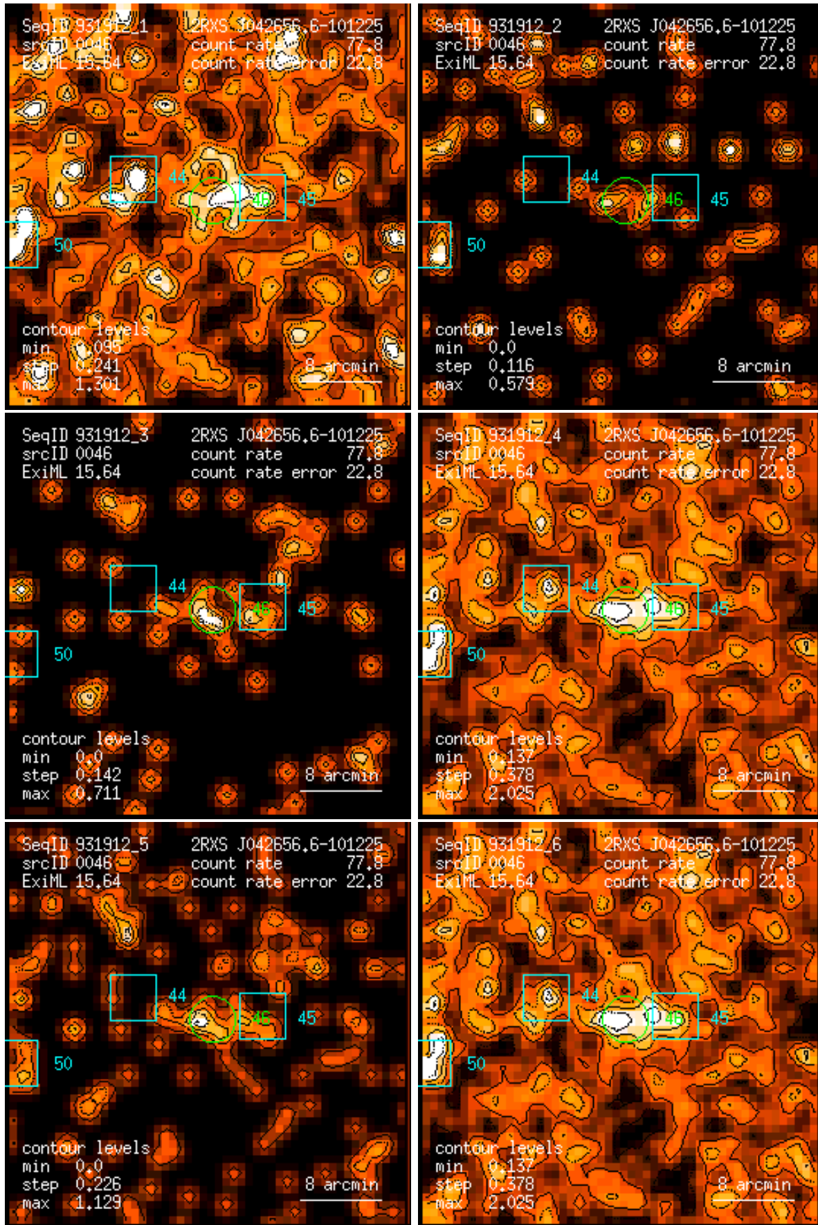
Figure 46: RASS 931912: detection 0046: band rate images, Gaussian filter: (1) PSPC channels 11 – 41, (2) 52 – 90, (3) 91 – 201, (4) 11 – 235, (5) 52 – 201, (6) 11 – 201. Broad band rates in counts/ks. Band rate contour levels in counts/ks/arcmin 2 .
