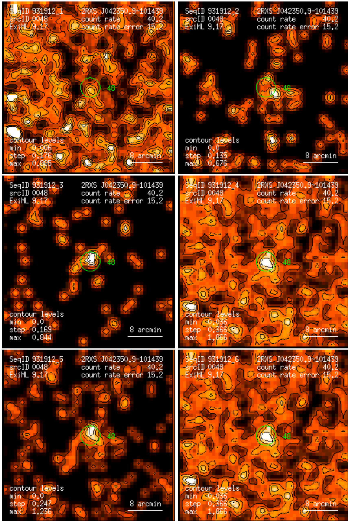
Figure 48: RASS 931912: detection 0048: band rate images, Gaussian filter: (1) PSPC channels 11 – 41, (2) 52 – 90, (3) 91 – 201, (4) 11 – 235, (5) 52 – 201, (6) 11 – 201. Broad band rates in counts/ks. Band rate contour levels in counts/ks/arcmin 2 .
