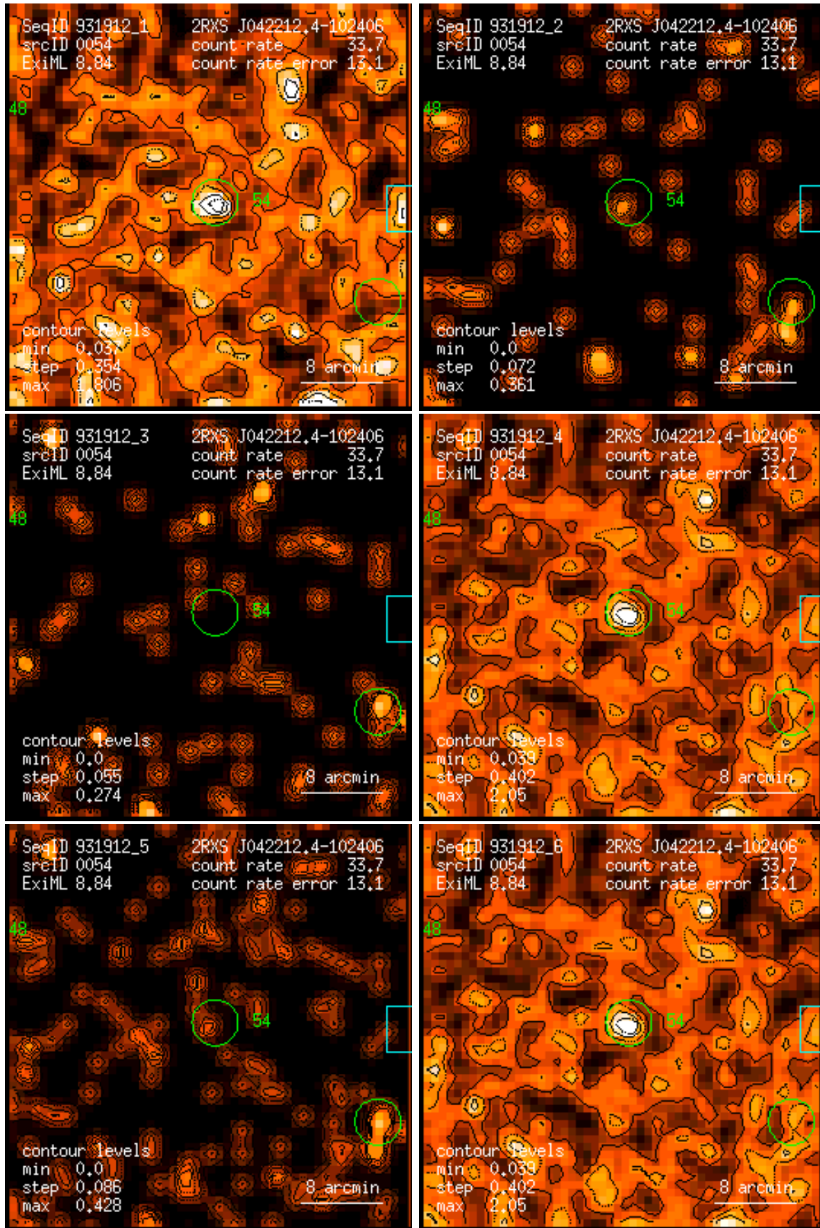
Figure 54: RASS 931912: detection 0054: band rate images, Gaussian filter: (1) PSPC channels 11 – 41, (2) 52 – 90, (3) 91 – 201, (4) 11 – 235, (5) 52 – 201, (6) 11 – 201. Broad band rates in counts/ks. Band rate contour levels in counts/ks/arcmin 2 .
