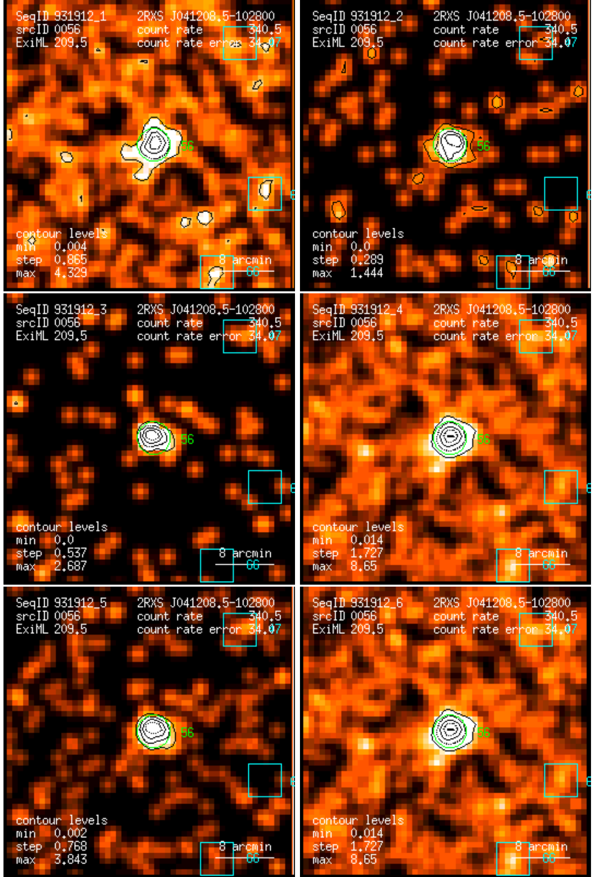
Figure 56: RASS 931912: detection 0056: band rate images, Gaussian filter: (1) PSPC channels 11 – 41, (2) 52 – 90, (3) 91 – 201, (4) 11 – 235, (5) 52 – 201, (6) 11 – 201. Broad band rates in counts/ks. Band rate contour levels in counts/ks/arcmin 2 .
