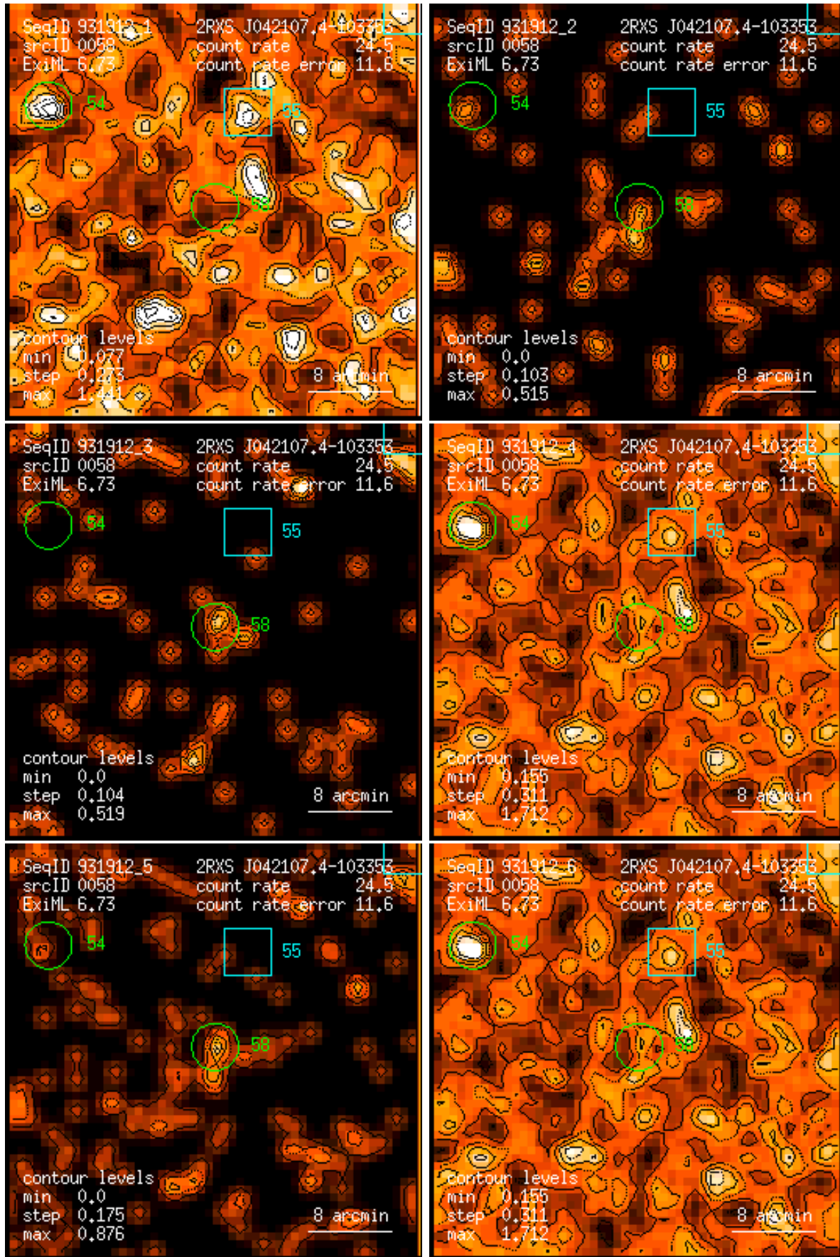
Figure 58: RASS 931912: detection 0058: band rate images, Gaussian filter: (1) PSPC channels 11 – 41, (2) 52 – 90, (3) 91 – 201, (4) 11 – 235, (5) 52 – 201, (6) 11 – 201. Broad band rates in counts/ks. Band rate contour levels in counts/ks/arcmin 2 .
