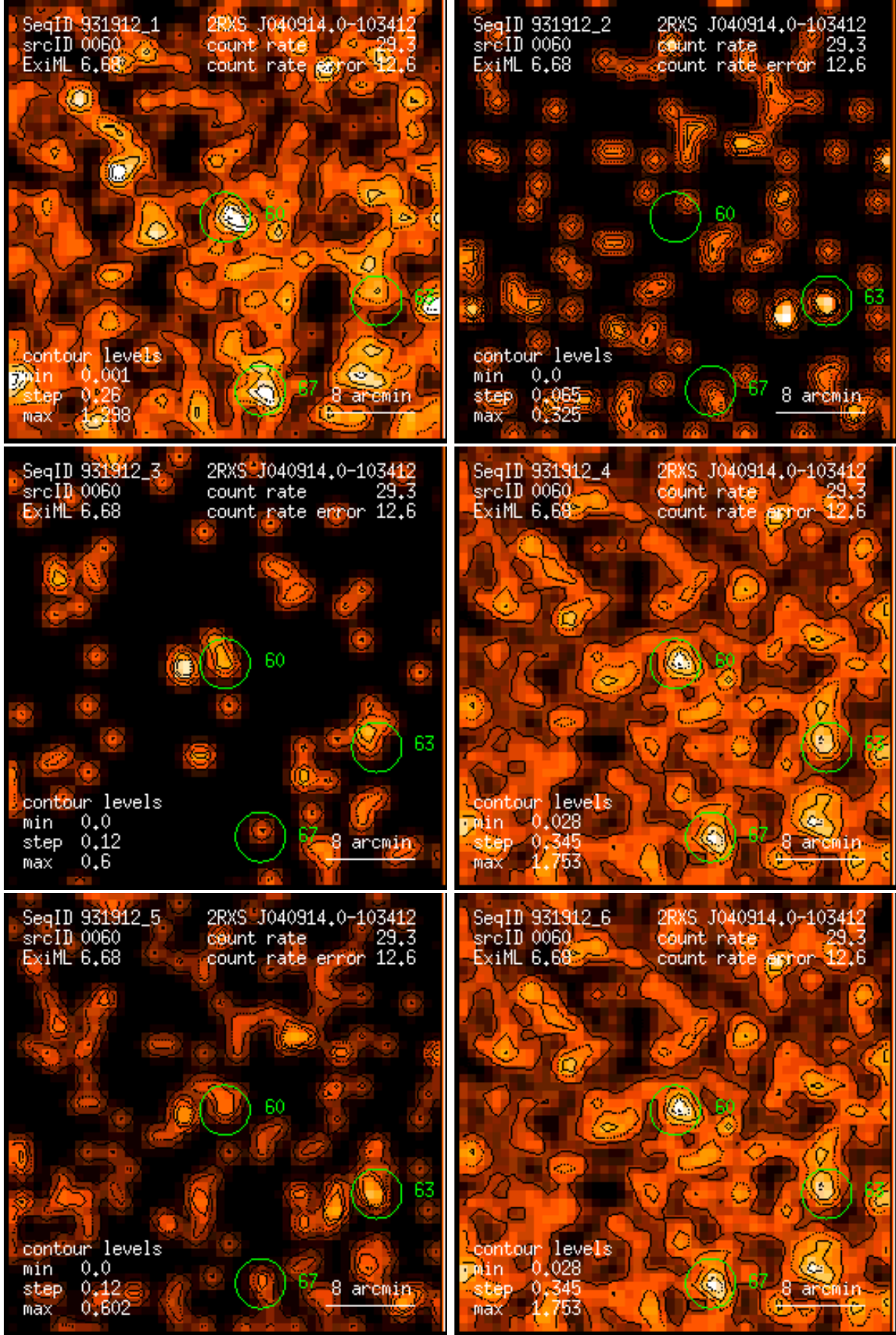
Figure 60: RASS 931912: detection 0060: band rate images, Gaussian filter: (1) PSPC channels 11 – 41, (2) 52 – 90, (3) 91 – 201, (4) 11 – 235, (5) 52 – 201, (6) 11 – 201. Broad band rates in counts/ks. Band rate contour levels in counts/ks/arcmin 2 .
