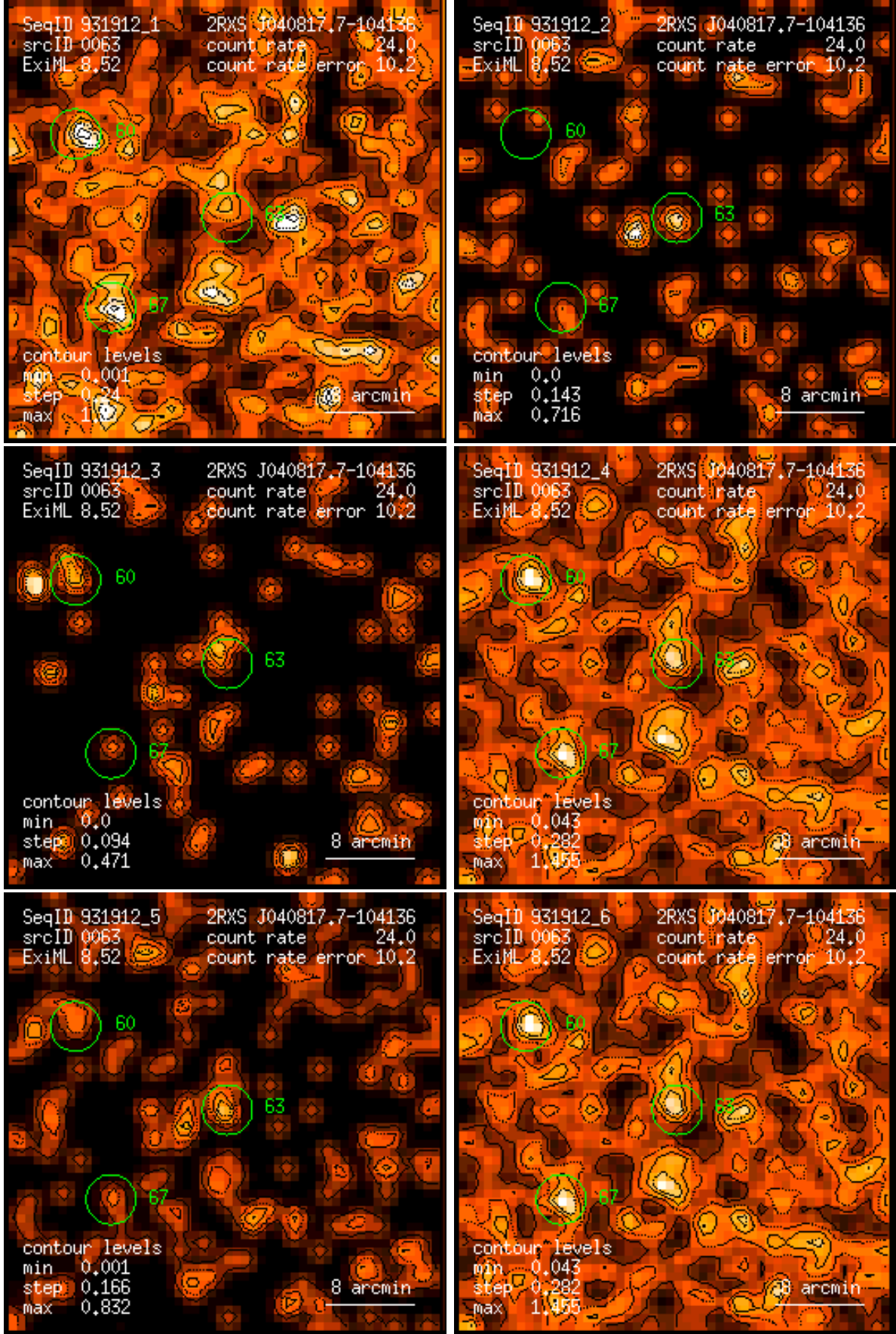
Figure 63: RASS 931912: detection 0063: band rate images, Gaussian filter: (1) PSPC channels 11 – 41, (2) 52 – 90, (3) 91 – 201, (4) 11 – 235, (5) 52 – 201, (6) 11 – 201. Broad band rates in counts/ks. Band rate contour levels in counts/ks/arcmin 2 .
